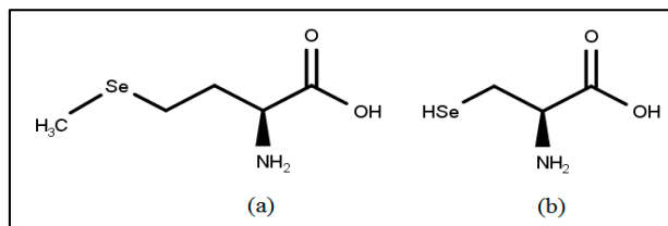
Figure 1. Chemical structures of (a) selenomethionine and (b) selenocysteine.
