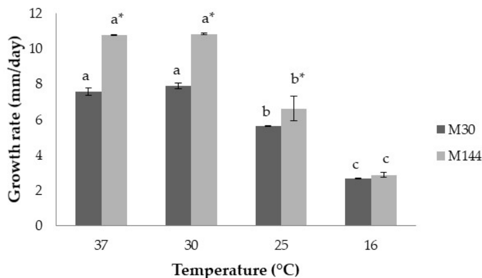
Figure 5. Growth rate (mm/day) of the Aspergillus flavus M144 and A. flavus M30 at the different temperatures studied over the 12 days incubation period. Different letters indicate significant differences at the different temperatures for the same strain ( p \leq 0.05 ). Asterisk (*) means significant differences between both strains at the same temperature ( p \leq 0.05 ).
