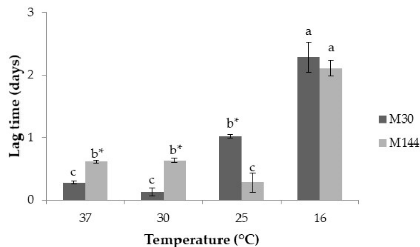
Figure 4. Lag time prior to growth (days) of the Aspergillus flavus M144 and A. flavus M30 at the different temperatures studied over the 12 days incubation period. Different letters indicate significant differences at the different temperatures for the same strain ( p \leq 0.05 ). Asterisk (*) means significant differences between both strains at the same temperature ( p \leq 0.05 ).
