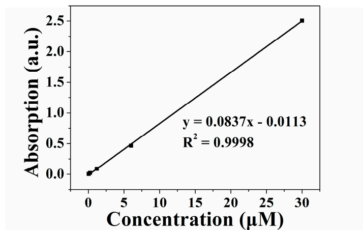
Figure S2. Standard curve of MB solution, showing the relationship between concentration and absorption.
