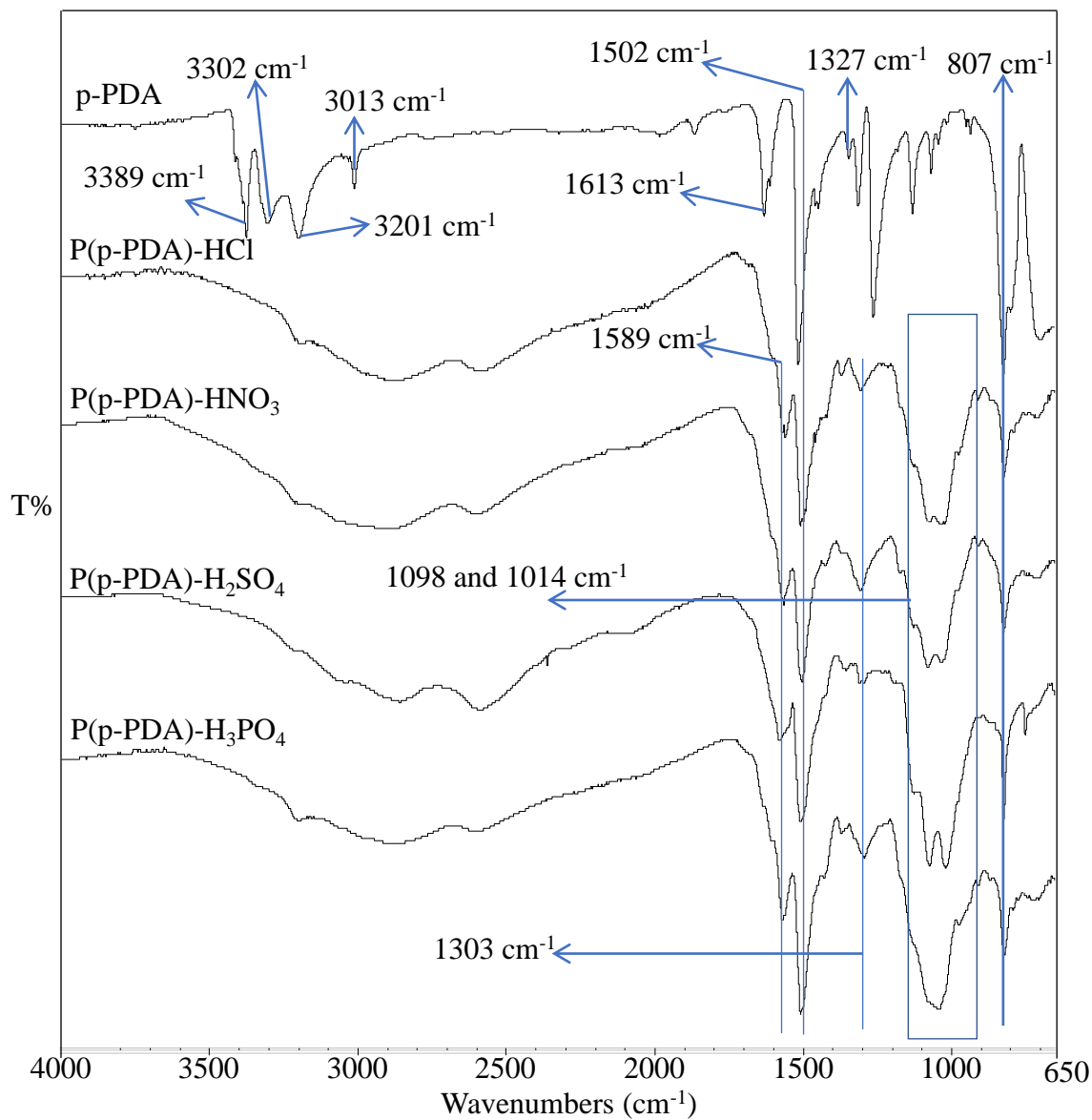
Figure S1: The FT-IR spectra of p(p-PDA) polymers doped with various types of acids.
