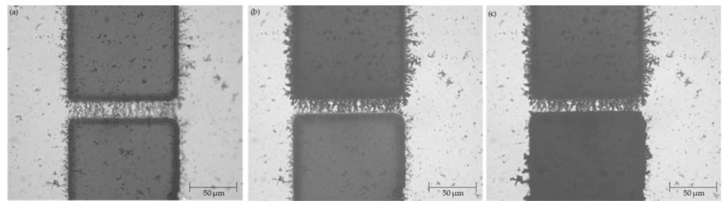
Figure 10. Results of PPy deposition over the CNT bridge spanning 20 \mu\text{m} electrode gap (a) prior to PPy application; (b) after the PPy deposition from the side of the top electrode reached roughly half-way through the CNT bridge and the polarity of the 0.9 Vpp DC bias was switched; (c) completion of PPy deposition over the CNT bridge.
