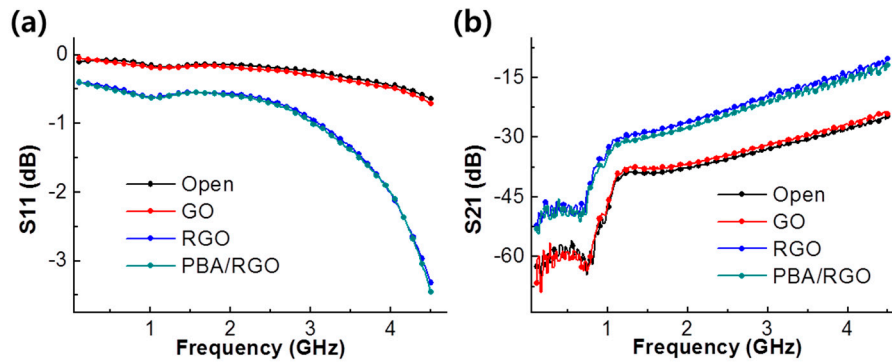
Figure S1. S-parameter results, (a) S11; (b) S21, of several electrodes with open without interconnector, GO, RGO, PBA/RGO.
