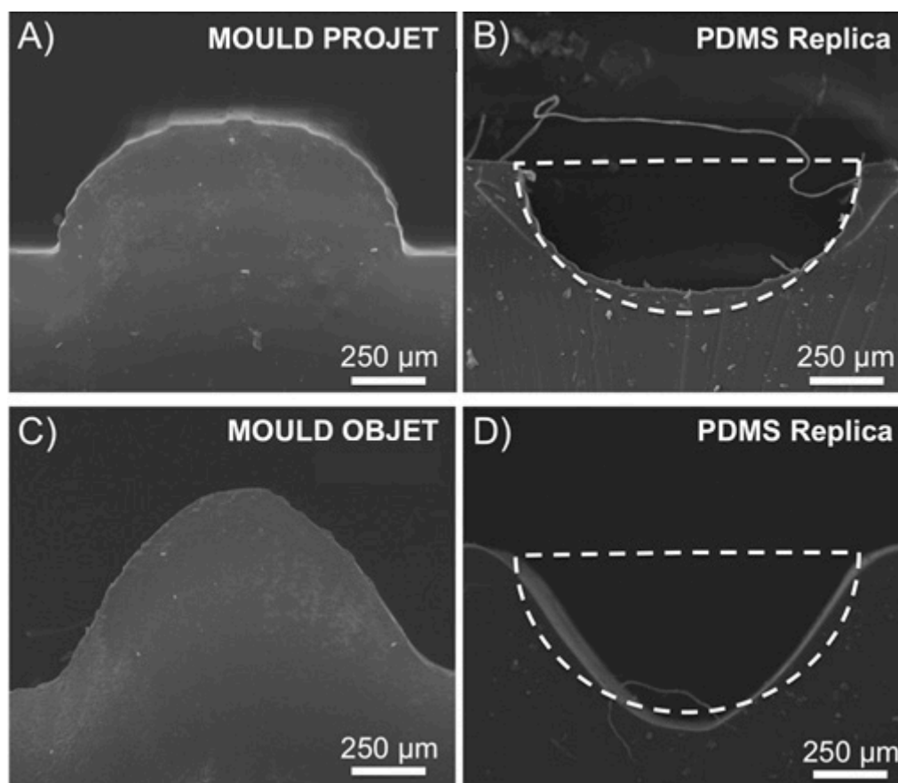
Figure S1. Physical characteristics of semi-circular positive relief patterns fabricated using additive manufacturing processes. (A) Pattern fabricated in VisJet Clear material using the ProJet 7000 HD system; (B) PDMS replica obtained from the master depicted in (A); (C) Pattern fabricated in Vero Clear using the Objet350 Connex system; (D) PDMS replica obtained from the master depicted in (C). Dotted lines represent the designed CAD geometry superimposed on SEM images of representative cross-sections.
