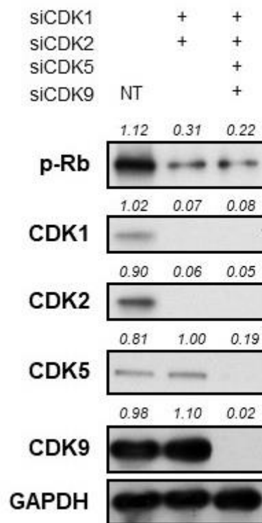
Figure S1. Western blot analysis results indicating the expression of various CDKs and their downstream molecules after transfection with siRNAs for 72 hours.
