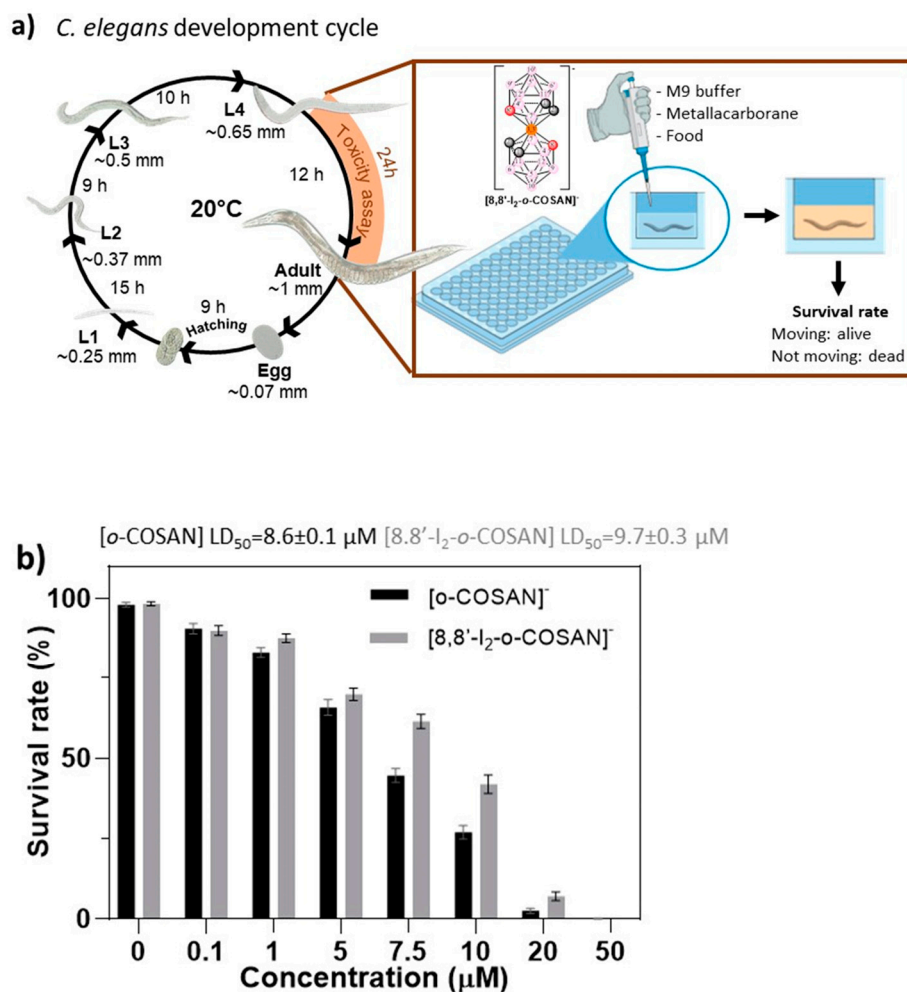
Figure 8. Toxicological evaluation of \text{Na}[o\text{-COSAN}] and \text{Na}[8,8'\text{-I}_2\text{-}o\text{-COSAN}] . (a) Schematic representation of C. elegans ' life cycle at 20^\circ\text{C} and exposure of the components from L4 stage to adult stage. (b) Survival rate of C. elegans after 24 h of exposure towards concentrations in a range 0–50 \mu\text{M} of \text{Na}[o\text{-COSAN}] (black) and \text{Na}[8,8'\text{-I}_2\text{-}o\text{-COSAN}] (grey).
