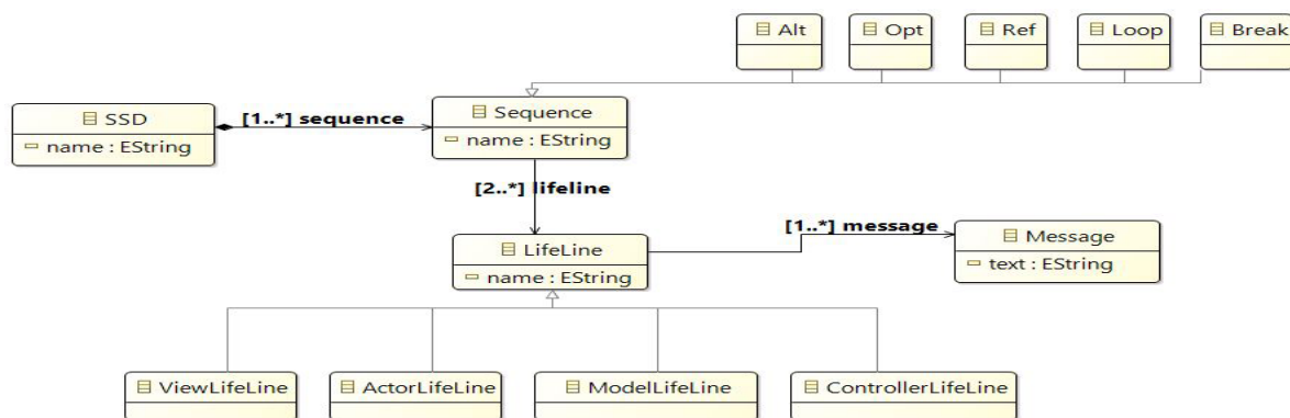
Figure 4. Main elements of the detailed sequence diagram in our approach.
