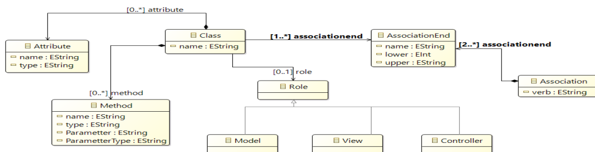
Figure 5. Main elements of the detailed class diagram in our approach.
