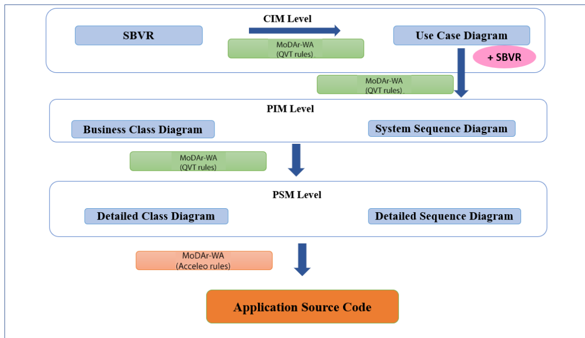
Figure 1. Overview of our model-driven architecture (MDA) transformational approach.
