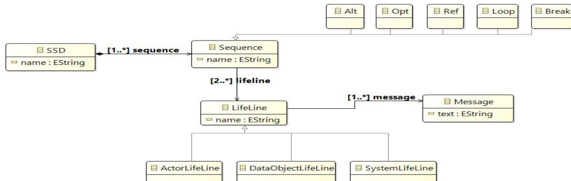
Figure 3. Main elements of the system sequence diagram in our approach.
