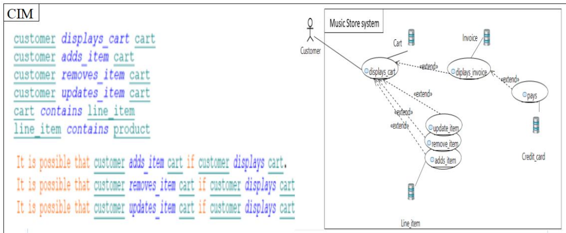
Figure 7. MoDAr-WA process and result of the music store system.
