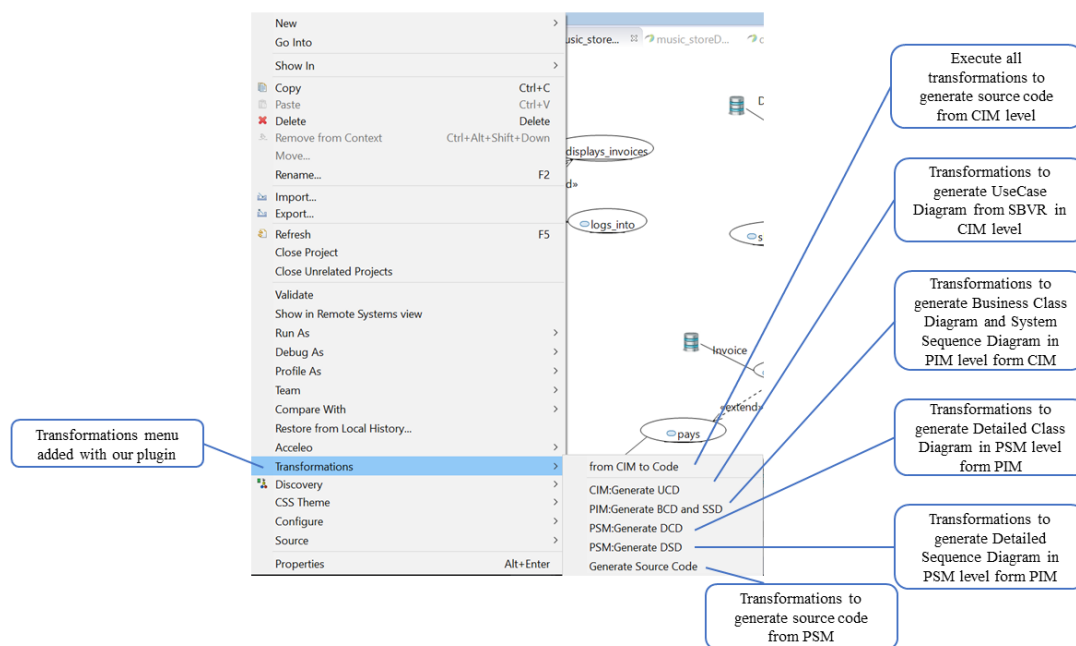
Figure 6. Transformation menu item of the model-driven architecture for web application (MoDar-WA) plug-in.
