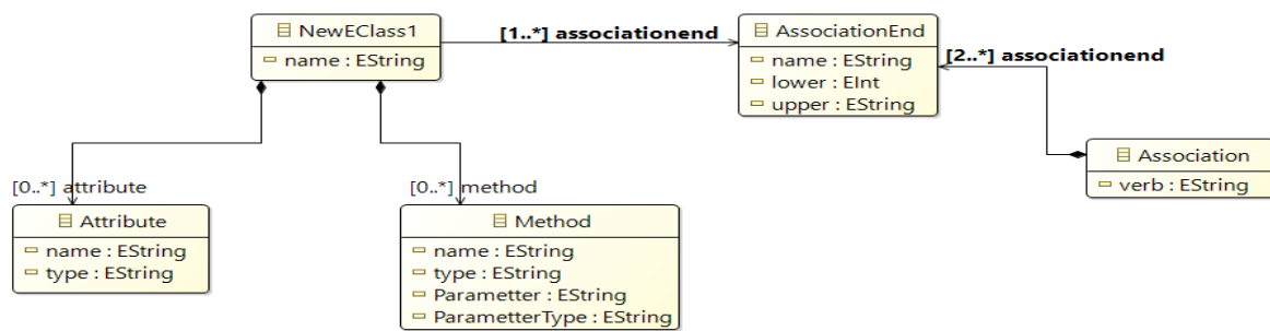
Figure 2. Main elements of the business class diagram in our approach.
