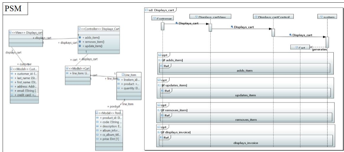
Figure 9. MoDar-WA process and result of the music store system.
