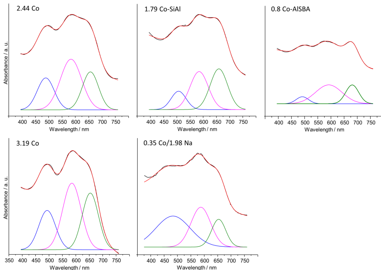
Figure S1. Deconvoluted UV-vis spectra measured in diffuse reflection mode at room temperature after heating the samples at 400°C in He for 30 min.
