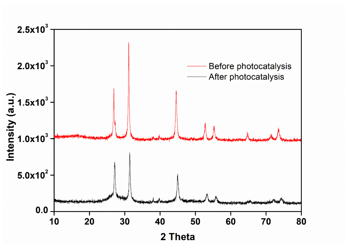
Figure S2. XRD patterns of NaBiS 2 before and after photocatalytic reaction.
