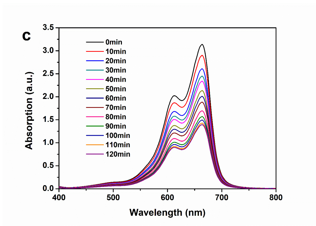
Figure S1. UV-vis absorption spectra curves of MB solution irradiated under (a) UV light; (b) visible light; (c) NIR light measured at interval times.
