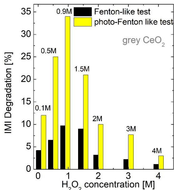
Figure S1. Effect of the H 2 O 2 concentration on the imidacloprid degradation after 3 hours with Fenton-like and photo-Fenton like tests utilizing the grey CeO 2 catalyst.
