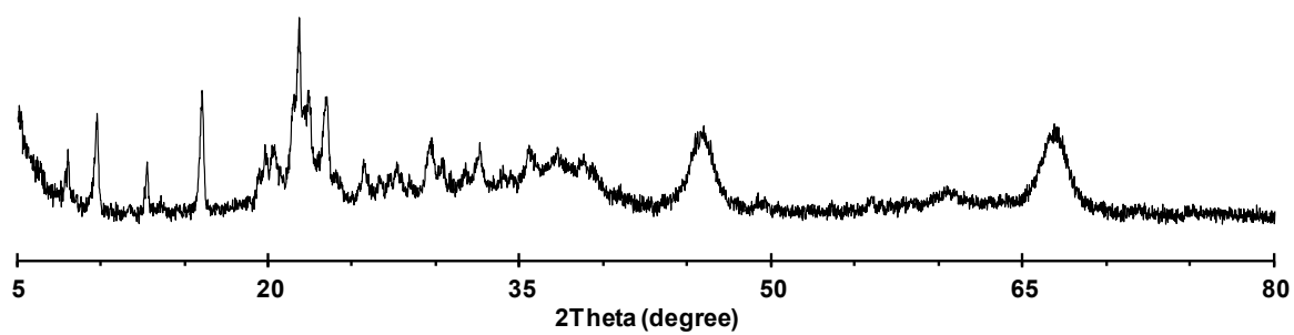
Fig. S1. XRD spectra of synthesized \text{Al}_2\text{O}_3 -SAPO-11 composite support
