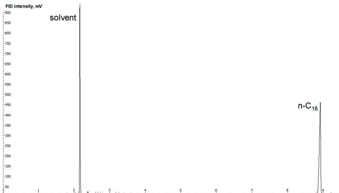
Fig. S3. Chromatogram of the feedstock n-C 16 in hexane.
