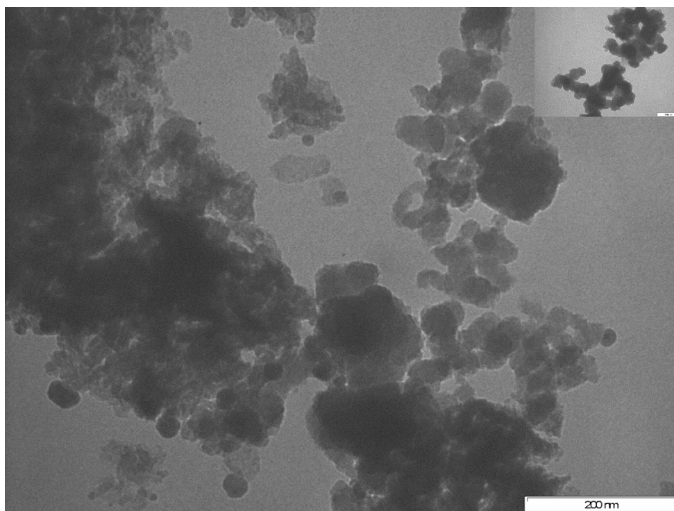
Figure S2: TEM images of Fe@Cu core-shell nanoparticles.
