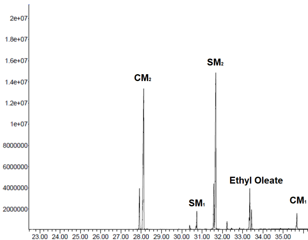
Figure S1: Representative chromatogram of the crude reaction mixture from the CM of 1 and 2 .
