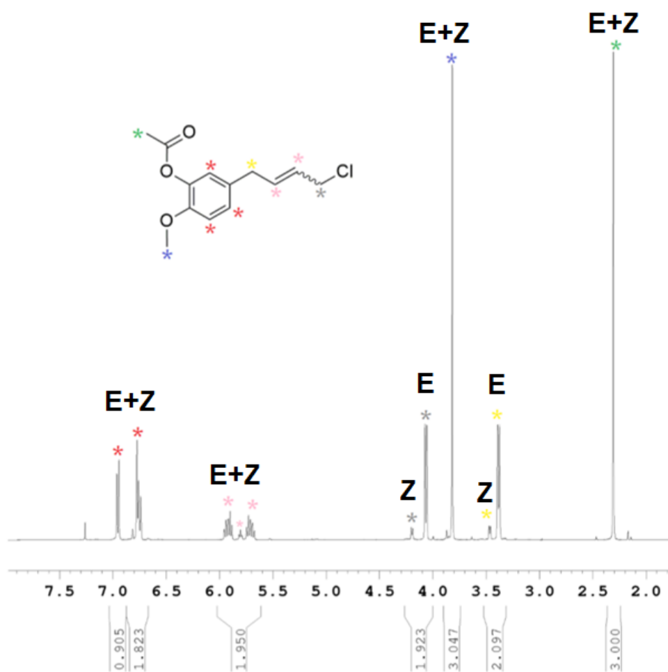
Figure S2: Representative 1 H NMR spectrum of the CM product from reaction of 3 and 4 (CDCl 3 , 400 MHz).
