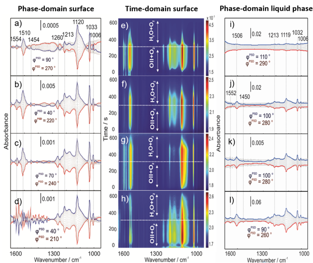
Figure 7. MES-ATR-IR spectra during Orange II concentration modulation over (a,e,i) Au-Fe(1:2)/TiO 2 , (b,f,j) Au-Fe(1:1)/TiO 2 , (c,g,k) Au-Fe(1:0.5)/TiO 2 , and (d,h,l) Au/TiO 2 .
