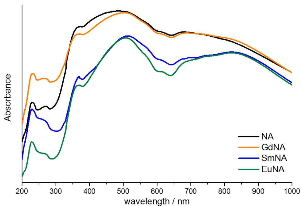
Figure S1. The UV-Vis-NIR absorption spectra of NA, SmNA, EuNA, and GdNA.
