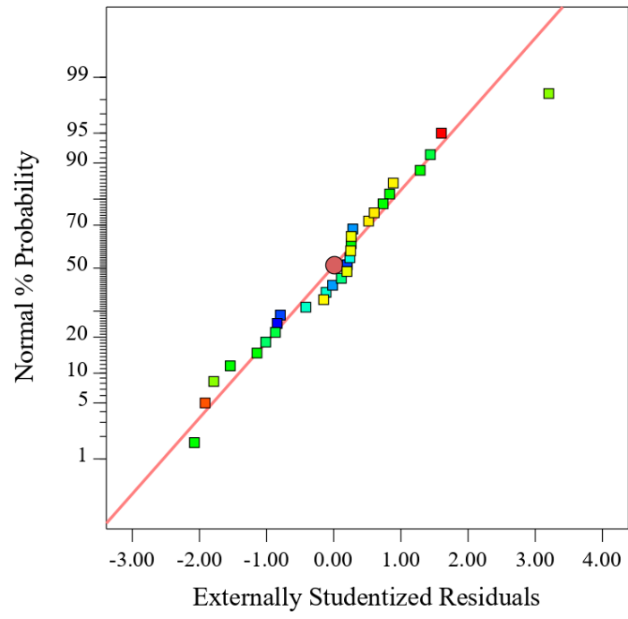
Figure S2. Residual plot for studentized residuals.
