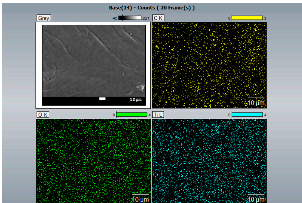
Figure S1. SEM-EDS mapping of synthesized electrodes.
