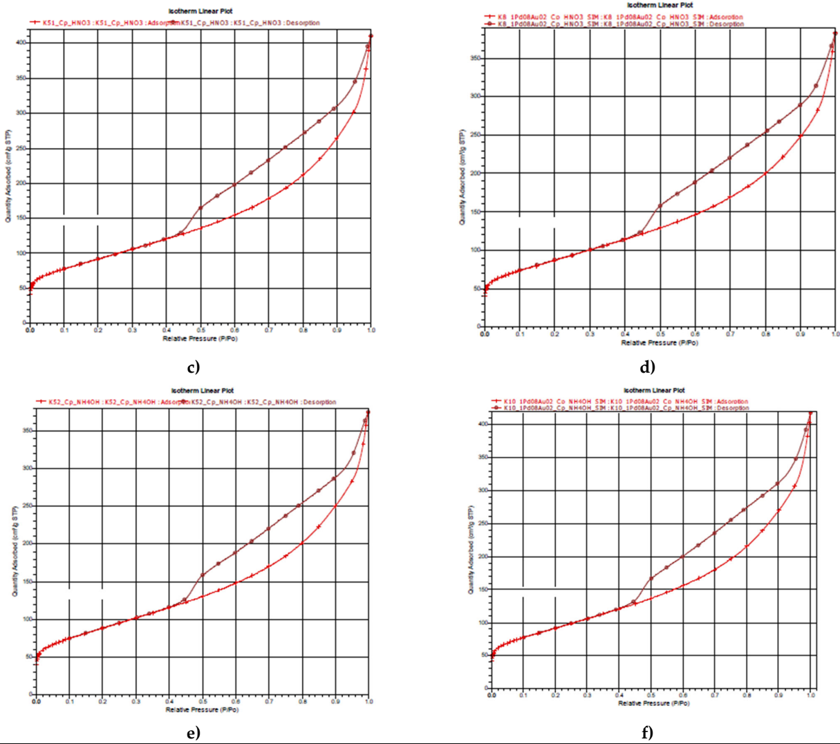
Figure 1. N_2 isotherms for Cp (a) and PdAu/Cp (b), Cp-HNO 3 (c) and PdAu/Cp-HNO 3 (d), Cp-NH 4 OH (e) and PdAu/Cp-NH 4 OH (f).
