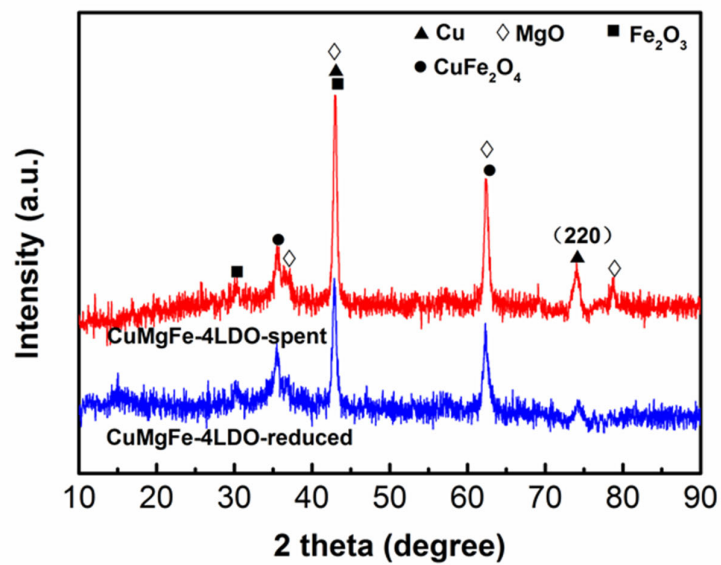
Figure S1. XRD patterns of the reduced and spent CuMgFe-4LDO catalysts.
