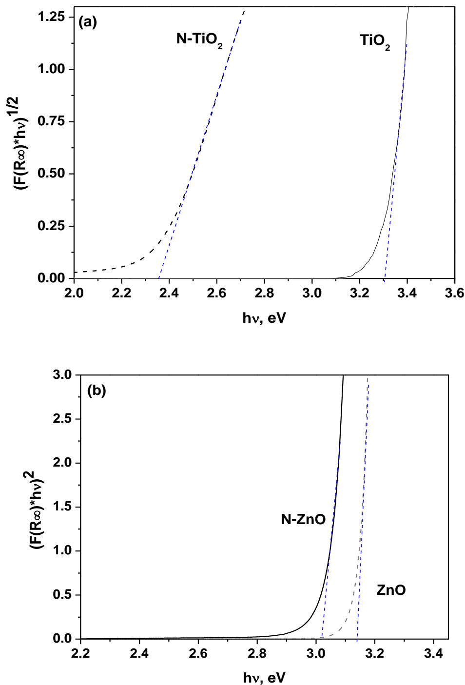
Figure 2. Band-gap estimation for (a) TiO 2 and N-TiO 2 , as well as (b) ZnO and N-ZnO samples.
