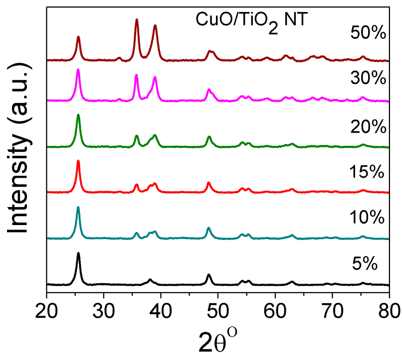
Figure S1. XRD patterns of CuO-TiO 2 nanotubes with different Cu content from 5–50 wt.%.
