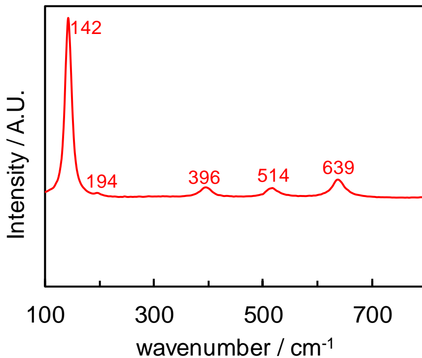
Figure S1. Raman spectra of the TiO 2 -impregnated a-silica tube. Reproduced from [9]. Copyright 2015, Catalysts.
