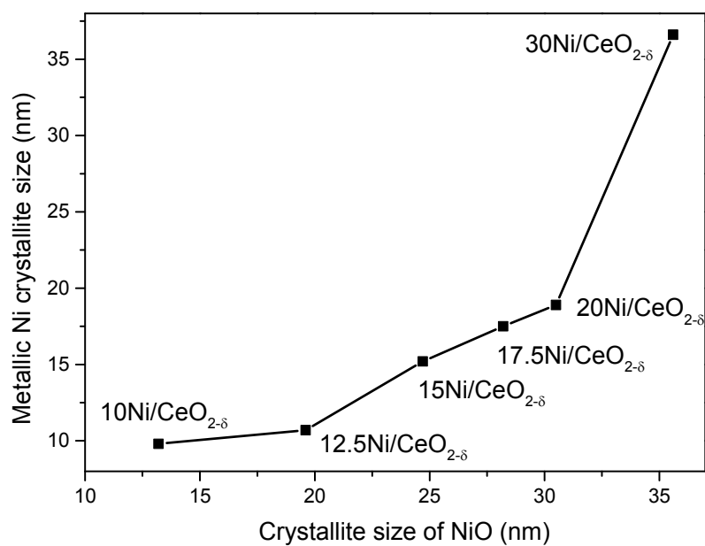
Figure S1. The dependence of metal crystallite sizes on those of metal oxides in the xNi/CeO 2-δ catalysts (x represents the loading amount (wt%) of Ni in the xNi/CeO 2-δ catalysts).
