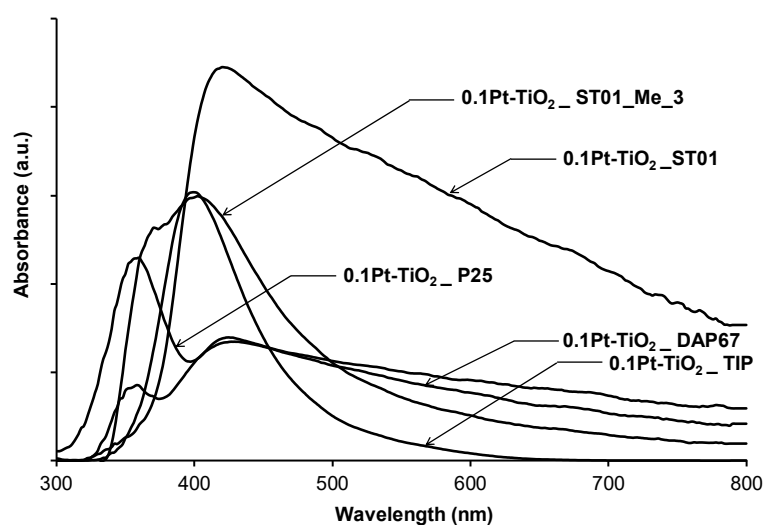
Figure 8. DR/UV-vis spectra of platinum-modified TiO 2 samples taken with bare TiO 2 supports as a reference.
