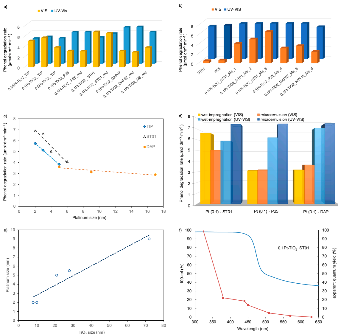
Figure 9. Photocatalytic activity for Pt-TiO 2 samples obtained by the wet-impregnation method (a), Pt-TiO 2 _Me samples obtained in w/o microemulsion system (b), Correlation between platinum particle size and photocatalytic activity of TIP, ST01 and DAP (c), Comparison of UV-vis and visible-light photocatalytic activity of Pt-modified samples based on ST01, P25 and DAP titania particles obtained using wet-impregnation and microemulsion methods (d), Correlation between platinum particle size and TiO 2 support particle size (e) and action spectrum of phenol oxidation on 0.1Pt-TiO 2 _ST01 (f).
