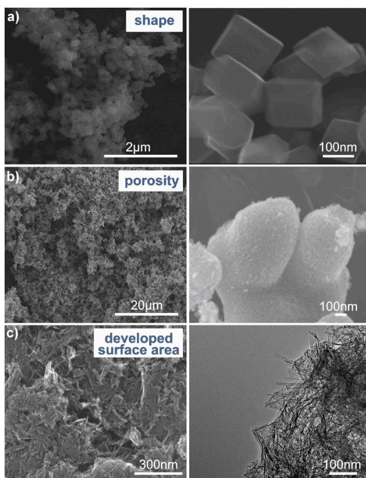
Figure 1. Microscopic images of bare decahedral anatase particles \text{TiO}_2\text{-DAP67} (a), \text{TiO}_2 nanospheres \text{TiO}_2\text{-NS} (b) and \text{TiO}_2 nanotubes \text{TiO}_2\text{-NT}_450 calcined at 450^\circ\text{C} (c).
