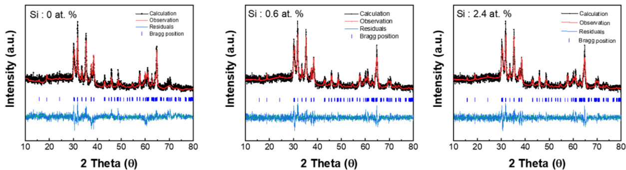
Figure S1. XRD analysis of \beta -Ga 2 O 3 nanofibers with different Si concentrations using Fullprof suite software.
