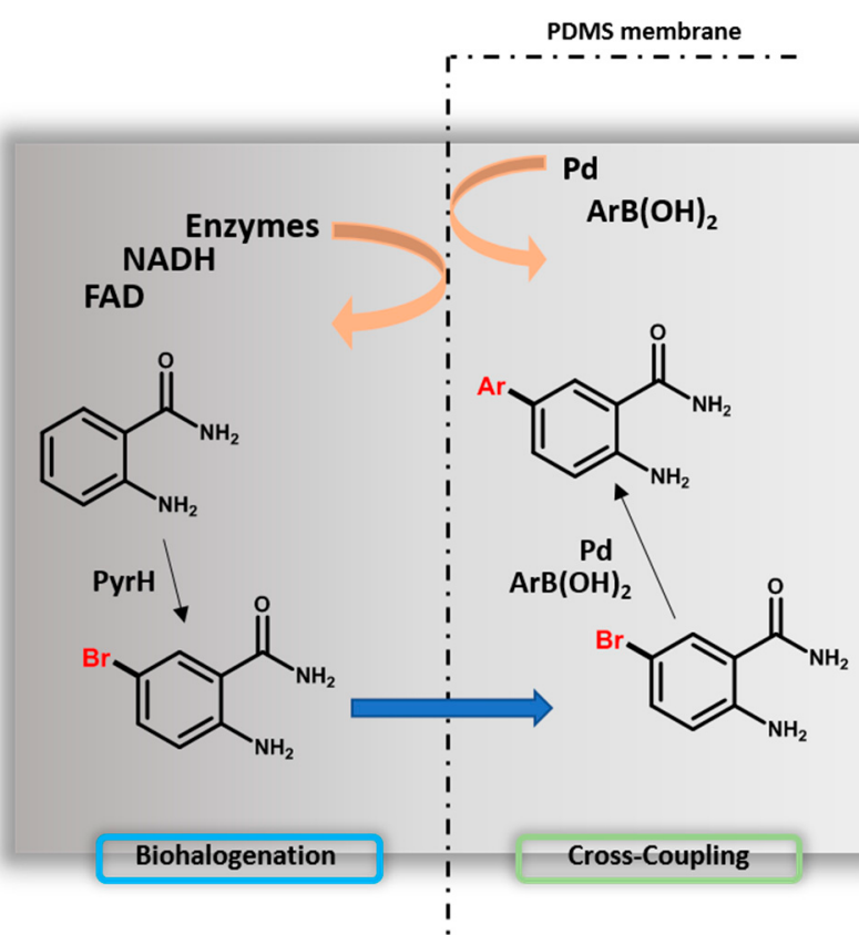
Figure 12. Polydimethylsiloxane (PDMS) compartmentalization. PDMS membrane permits diffusion of non-polar compounds (substrates, intermediates), while polar compounds such as enzymes, Pd catalysts, and cofactors are blocked. This compartmentalization overcomes the incompatibility of the enzyme and transition metal that reduces the efficiency of the chemoenzymatic process. Figure adapted from [5].
