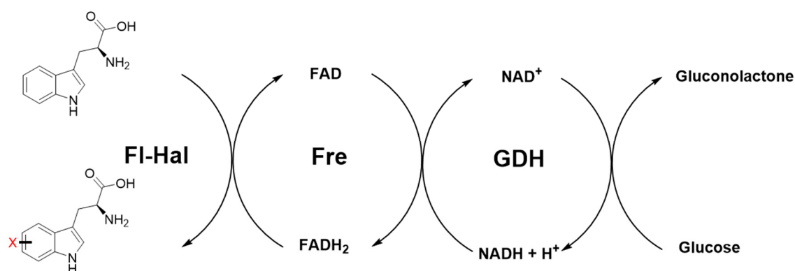
Figure 4. For the regeneration of \text{FADH}_2 , which is needed for the production of the reactive species hypohalous acid, two auxiliary enzymes can be used: a flavin reductase (Fre) for the reduction of FAD and a glucose dehydrogenase for the reduction of \text{NAD}^+ . Overall, the co-substrate glucose is used in excess, whereas the more expensive cofactors FAD and \text{NAD}^+ can be recycled.
