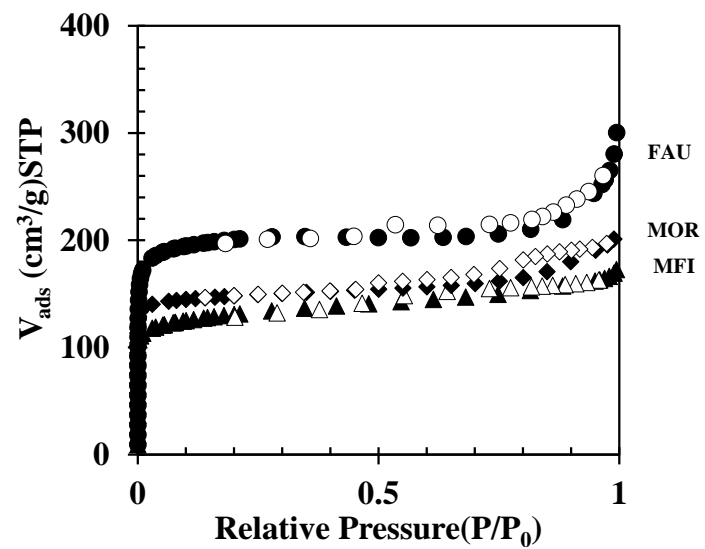
Figure S1: N 2 adsorption (solid symbols) and desorption (open symbols) isotherms at 77 K of FAU, MOR and MFI zeolites.
