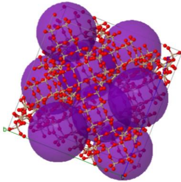
FAU (purple ball = supercage)
