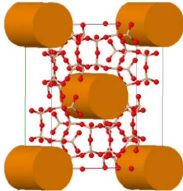
MOR (cylinder: large channel)
