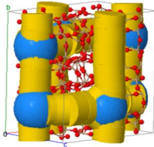
MFI: blue ball: intersection channel (yellow cylinder)
