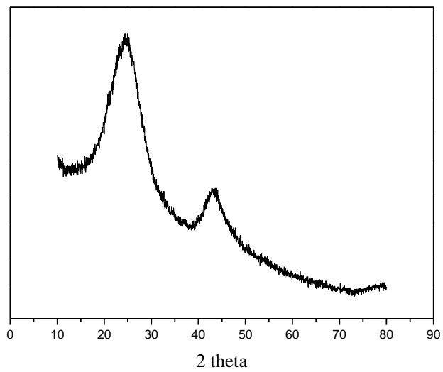
Figure S2. The XRD pattern of high dispersed PdCl 2 on Pd/C treated with aqua regia.
