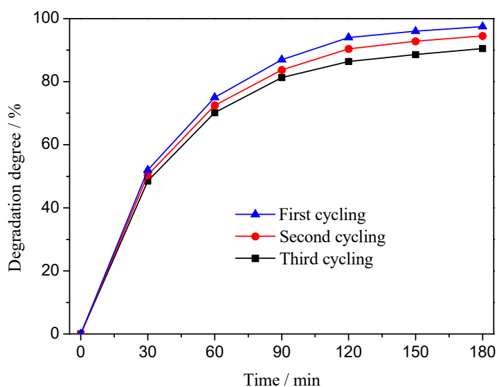
Fig. S1 Photocatalysis for HBCD degradation in the UV/TiO 2 /KPS system with three time cycling uses.
