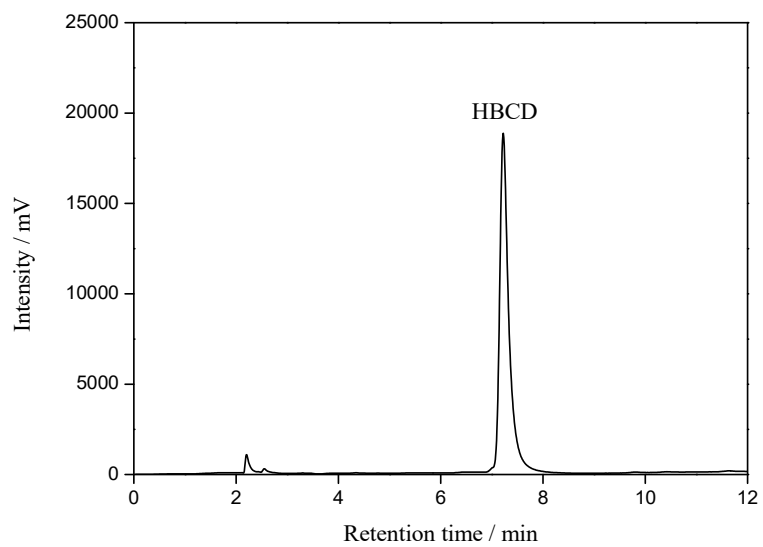
Fig. S2 The HPLC chromatogram of HBCD.
