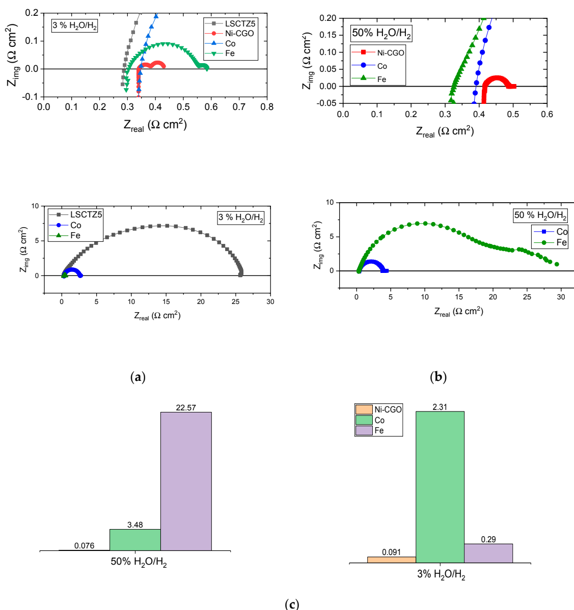
Figure 4. Electrochemical impedance spectroscopy (EIS) data Nyquist plot from Ni-CGO-, Co- and Fe-infiltrated LSCTZ5 at 750 °C in (a) 3% H 2 O/H 2 and (b) 50% H 2 O/H 2 ; the high frequency intercept is magnified in a separate (c) bar graph plot for comparison with R_p values given in Ω cm 2 .
