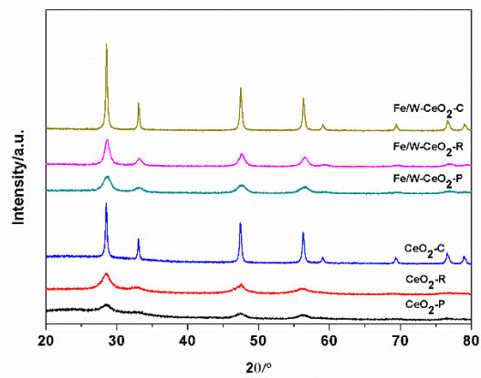
Figure S1. XRD patterns of Fe/W-CeO 2 and CeO 2 catalysts.
