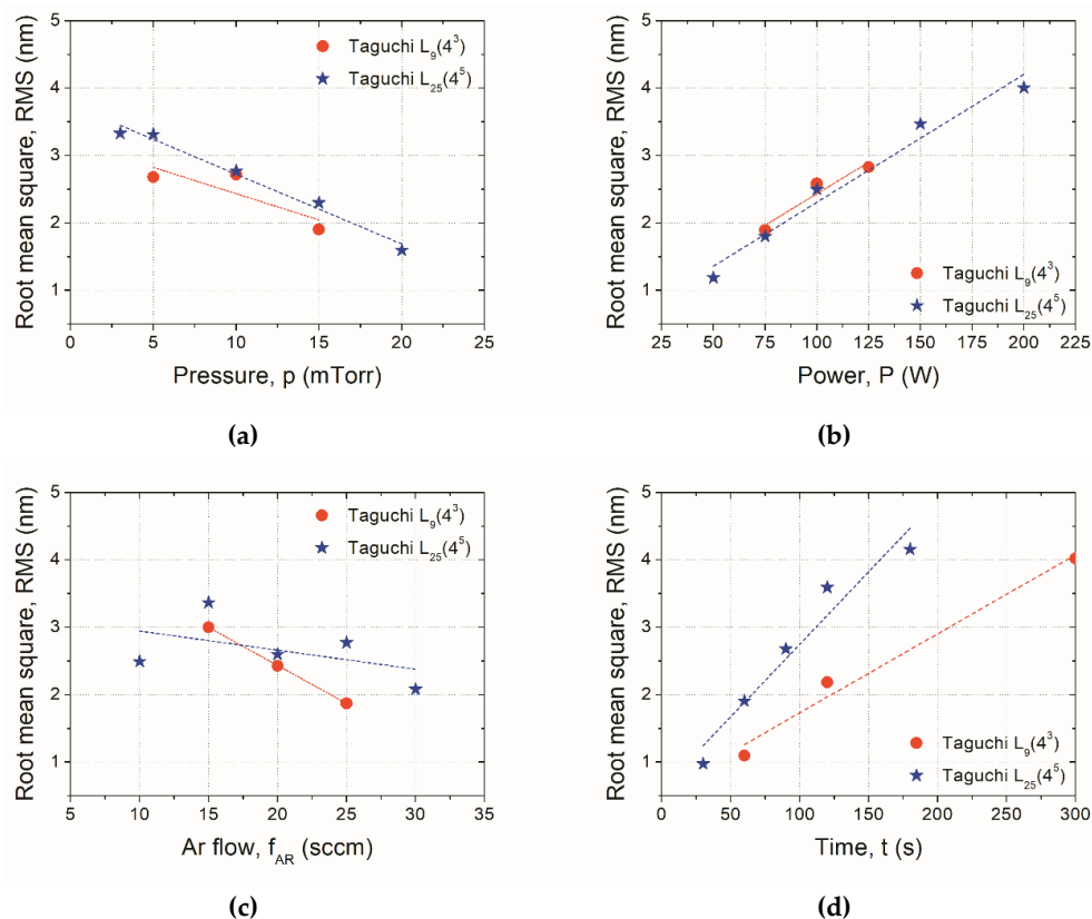
Figure 3. Influence of magnetron sputtering process' parameters onto roughness of aluminum films: (a) pressure in the reactive chamber, (b) DC power applied to the electrodes, (c) argon flow, and (d) time of the process.
