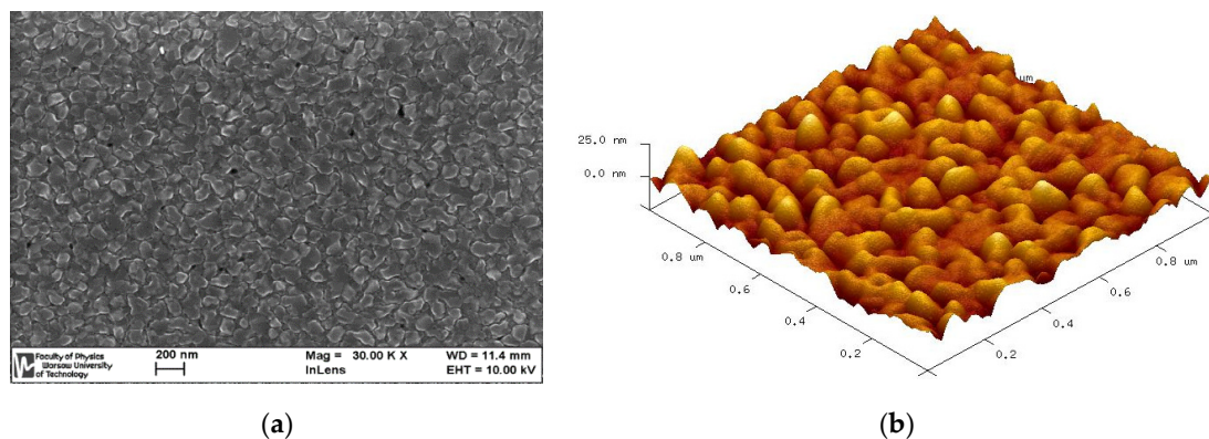
Figure 1. Surface topography of 30 nm Al films sputtered using pulsed-DC magnetron sputtering process: (a) HR-SEM, and (b) AFM micrographs.
