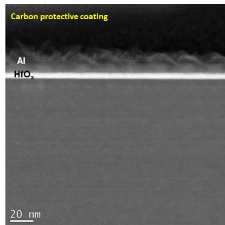
Figure 2. The cross-section (HR-TEM, Z-contrast) of Al/HfO x stack fabricated on a silicon substrate using a pulsed-DC magnetron sputtering process.
