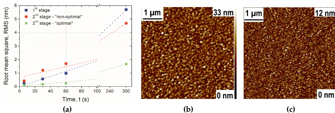
Figure 4. (a) Comparison of the roughness level of aluminum films fabricated using investigated sputtering procedures, and AFM micrographs of Al surface after formation using (b) ‘non-optimal’ (RMS = 4.8 nm), and (c) ‘optimal’ (RMS = 1.7 nm) recipe; sputtering time = 300 s.
