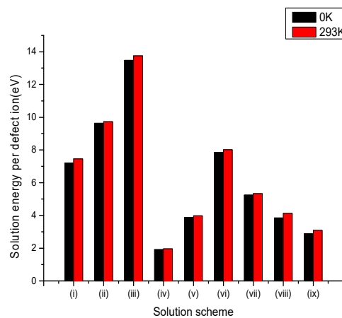
Figure 4. Bar chart of solution energies vs. solution schemes for tetravalent dopant ( V^{4+} ) at the Li and Nb sites, considering the first neighbours in relation to the c axis.
