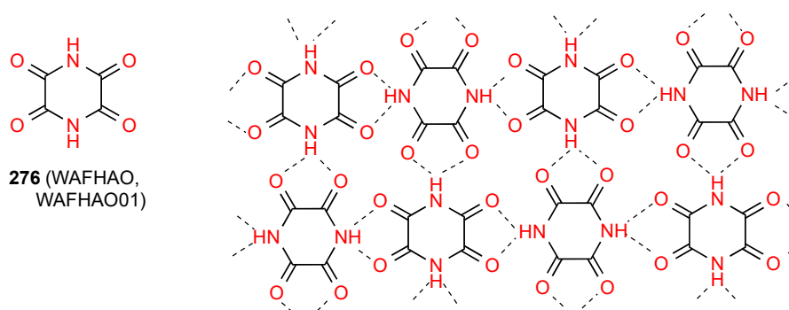
Figure 78. Structure adopted by compound 276.
