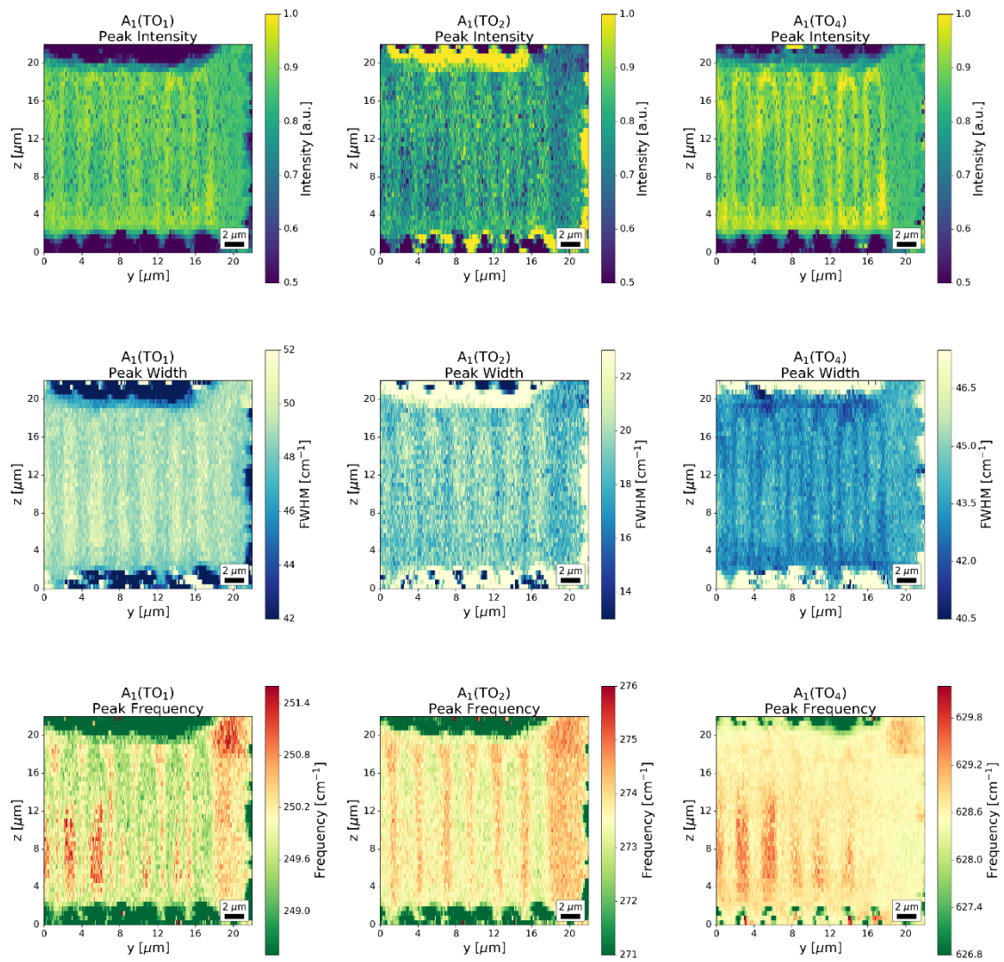
Figure S1 Complete set of colormaps generated from frequencies, intensities and peak widths of the analyzed A_1(\text{TO}) phonon modes in TFLN.
