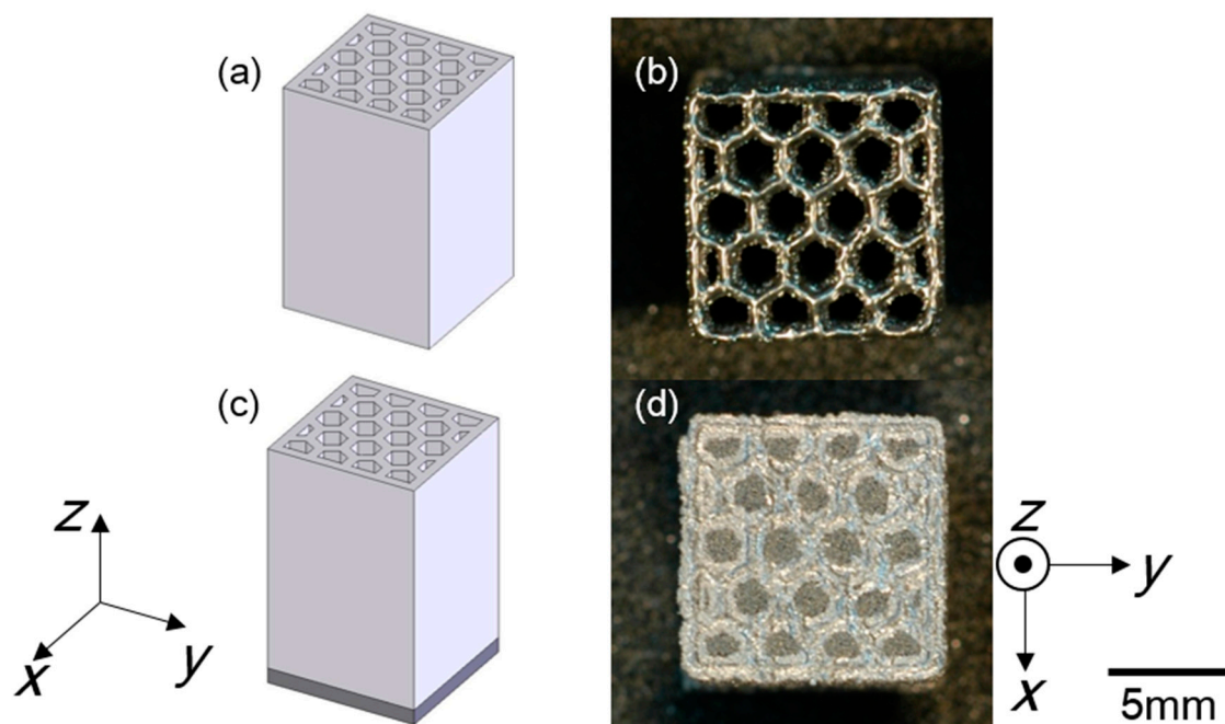
Figure 1. Three dimensional image of CAD model and pictures of specimen top surface for (a,b) porous specimen with elongated honeycomb pores and (c,d) powder/solid composite with un-melted powder particles within the pores (composite specimen).
