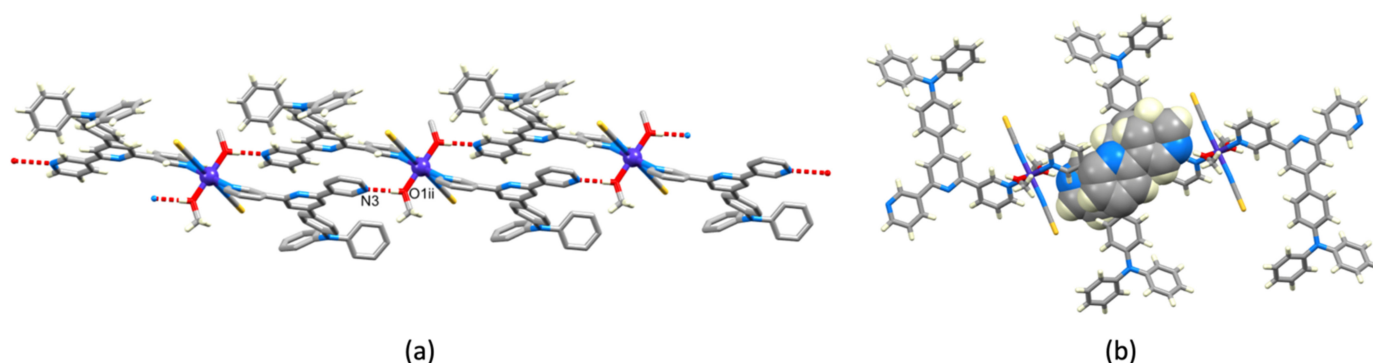
Figure 10. (a) Part of one hydrogen-bonded 1D-chain in [\text{Co}(\text{NCS})_2(\mathbf{2})_2(\text{MeOH})_2] \cdot 3\text{CHCl}_3 (symmetry code ii = 1 - x, -y, 1 - z ), and (b) the \pi -stacking interaction between pairs of terpyridine units within the chain.
