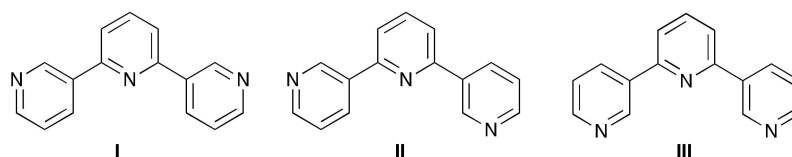
Scheme 1. Limiting planar conformations of 3,2':6',3''-tpy.
