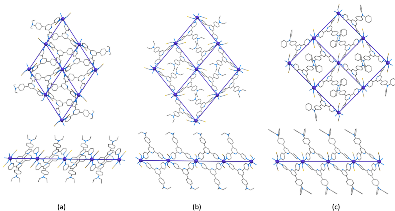
Figure 6. The (4,4) net ( top ) and a view down the b -axis ( bottom ) in (a) [\text{Co}(\text{NCS})_2(\mathbf{1})]_n \cdot 0.8n\text{CHCl}_3 , (b) [\text{Co}(\text{NCS})_2(\mathbf{3})]_n \cdot 2n\text{CHCl}_3 , and (c) [\text{Co}(\text{NCS})_2(\mathbf{4})]_n . The Co...Co vectors are depicted as blue lines to aid visualization of the (4,4) nets.
