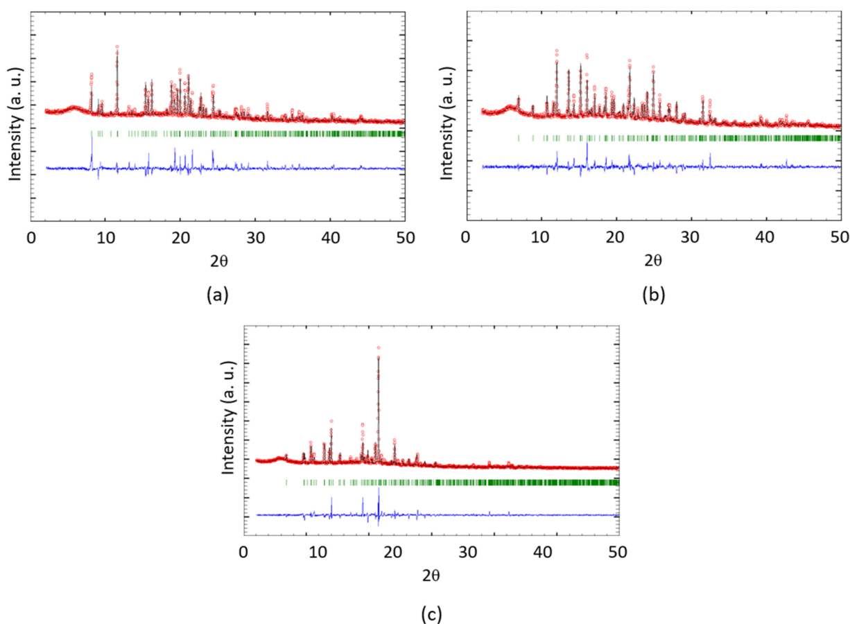
Figure 8. PXRD (CuK \alpha 1 radiation) patterns for (a) [\text{Co}(\text{NCS})_2(1)]_n \cdot 0.8n\text{CHCl}_3 , (b) [\text{Co}(\text{NCS})_2(3)]_n \cdot 2n\text{CHCl}_3 , and (c) [\text{Co}(\text{NCS})_2(4)]_n up to 2\theta = 50^\circ . The experimental pattern (red circles) is compared with the best fit from the Rietveld refinement analysis (black line). Bragg peak positions (green) and differences between the calculated and experimental plots (blue) are shown.
