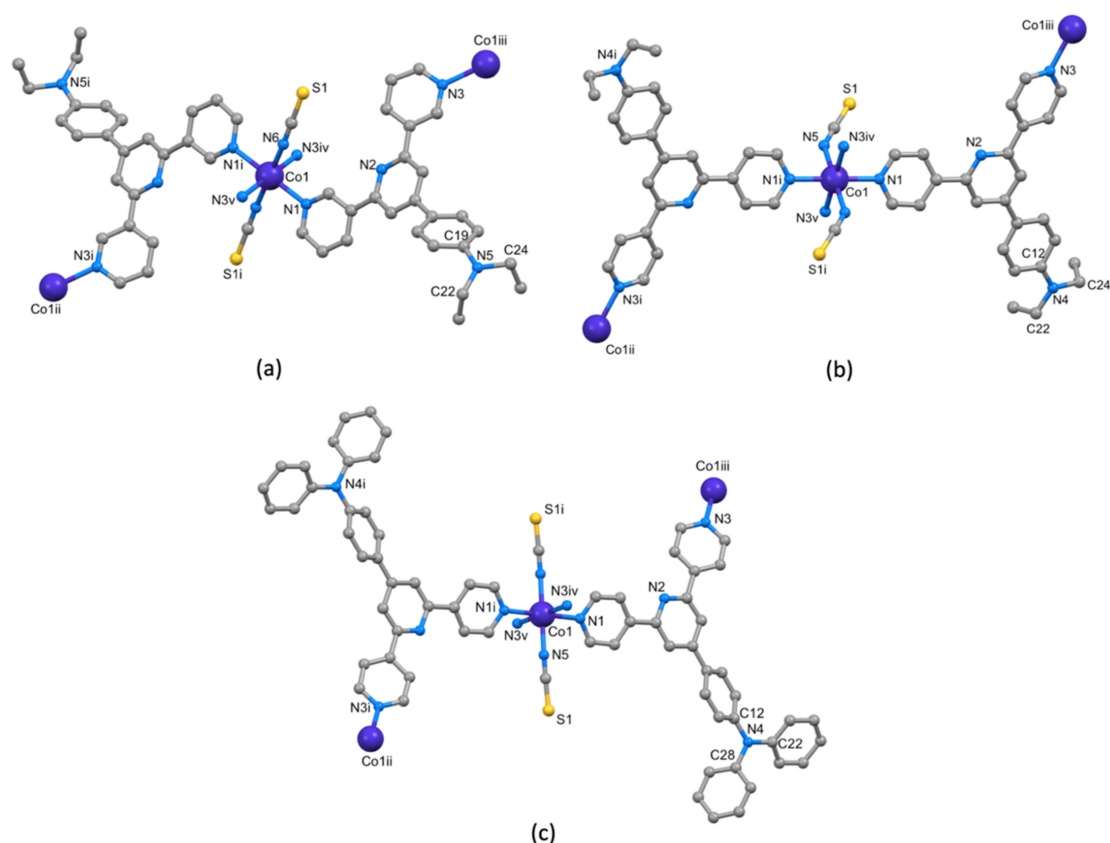
Figure 4. Structures of the repeat units in (a) [\text{Co}(\text{NCS})_2(\mathbf{1})]_n \cdot 0.8n\text{CHCl}_3 (symmetry codes: i = -x, 2 - y, 1 - z ; ii = -1/2 - x, 1/2 + y, 1/2 - z ; iii = 1/2 - x, -1/2 + y, 3/2 - z ; iv = 1/2 - x, 1/2 + y, 3/2 - z ; v = -1/2 + x, 3/2 - y, -1/2 + z ), (b) [\text{Co}(\text{NCS})_2(\mathbf{3})]_n \cdot 2n\text{CHCl}_3 (symmetry codes: i = 2 - x, 2 - y, 1 - z ; ii = 3/2 - x, 1/2 + y, 1/2 - z ; iii = 5/2 - x, -1/2 + y, 3/2 - z ; iv = 5/2 - x, 1/2 + y, 3/2 - z ; v = -1/2 + x, 3/2 - y, -1/2 + z ), and (c) [\text{Co}(\text{NCS})_2(\mathbf{4})]_n (symmetry codes: i = 1 - x, 1 - y, 1 - z ; ii = 1 - x, -1/2 + y, 1/2 - z ; iii = 1 - x, 1/2 + y, 3/2 - z ; iv = x, 3/2 - y, -1/2 + z ; v = 1 - x, -1/2 - y, 3/2 + z ).
