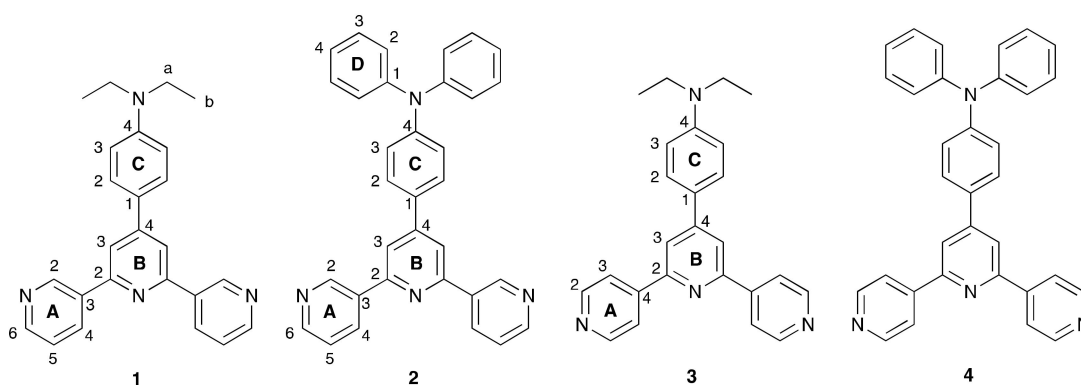
Scheme 2. Structures of ligands 1–4, with atom labelling, used for NMR spectroscopic assignments of 1, 2, and 3. The NMR spectroscopic data for 4 have previously been reported [8,15].
