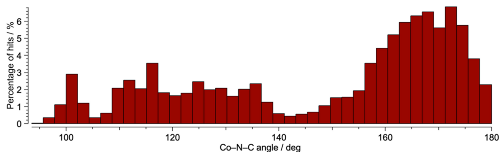
Figure 5. Distribution of Co–N NCS –C NCS bond angles in compounds containing N -bonded thiocyanate ligands coordinated to cobalt(II) found in the CSD (version 2022.1.0).
