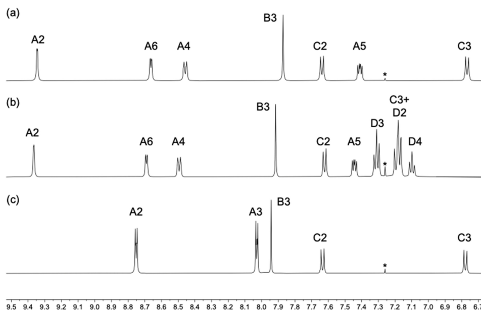
Figure 1. The aromatic regions in the ^1H NMR spectra of (a) 1, (b) 2, and (c) 3 (500 MHz, 298 K, CDCl_3 ). * = residual CHCl_3 . Scale: \delta /ppm. Atom labelling is defined in Scheme 2.
