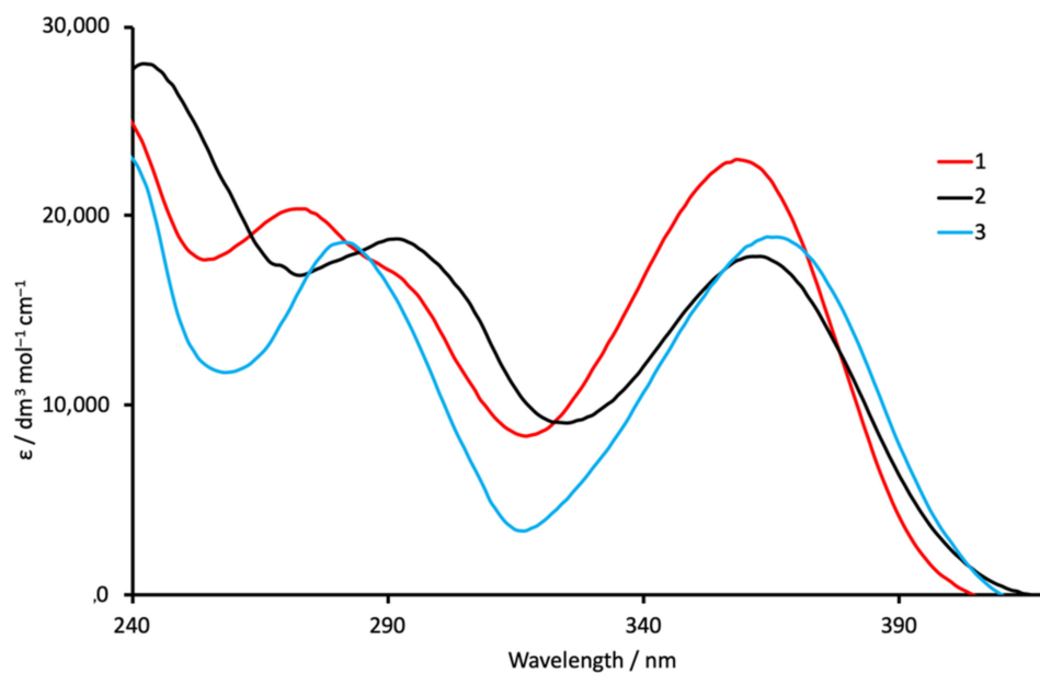
Figure 2. Solution absorption spectra of compounds 1–3 ( CH_2Cl_2 , 2 \times 10^{-5} \text{ mol dm}^{-3} ).
