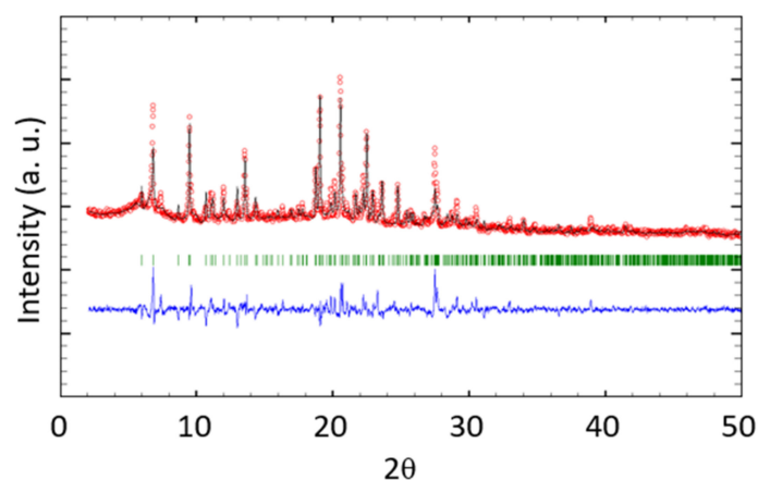
Figure 11. PXRD (CuK \alpha 1 radiation) patterns for [Co(NCS) _2 (2) _2 (MeOH) _2 ] \cdot 3CHCl _3 up to 2\theta = 50^\circ . The experimental pattern (red circles) is matched with the best fit from the Rietveld refinement analysis (black line). Bragg peak positions (green) and differences between the calculated and experimental plots (blue) are also shown. See Figure S30 for the complete PXRD.
