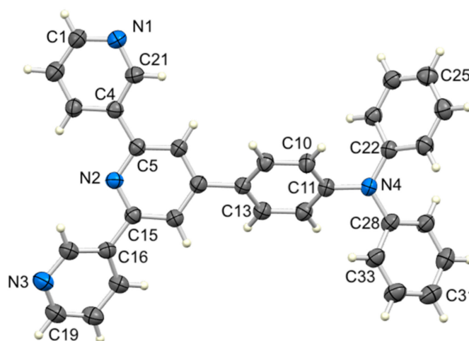
Figure 3. The structure of ligand 2 with ellipsoids plotted at a 40% probability level.
