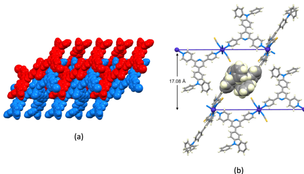
Figure 7. (a) Packing of adjacent sheets in the crystal lattice of [\text{Co}(\text{NCS})_2(\mathbf{4})]_n (viewed down the b -axis). (b) Pairs of 4-( N,N -diphenylamino)phenyl groups (space-filling representation) in non-adjacent sheets engage in an embrace; 17.08 Å = twice the inter-plane separation of adjacent sheets.
