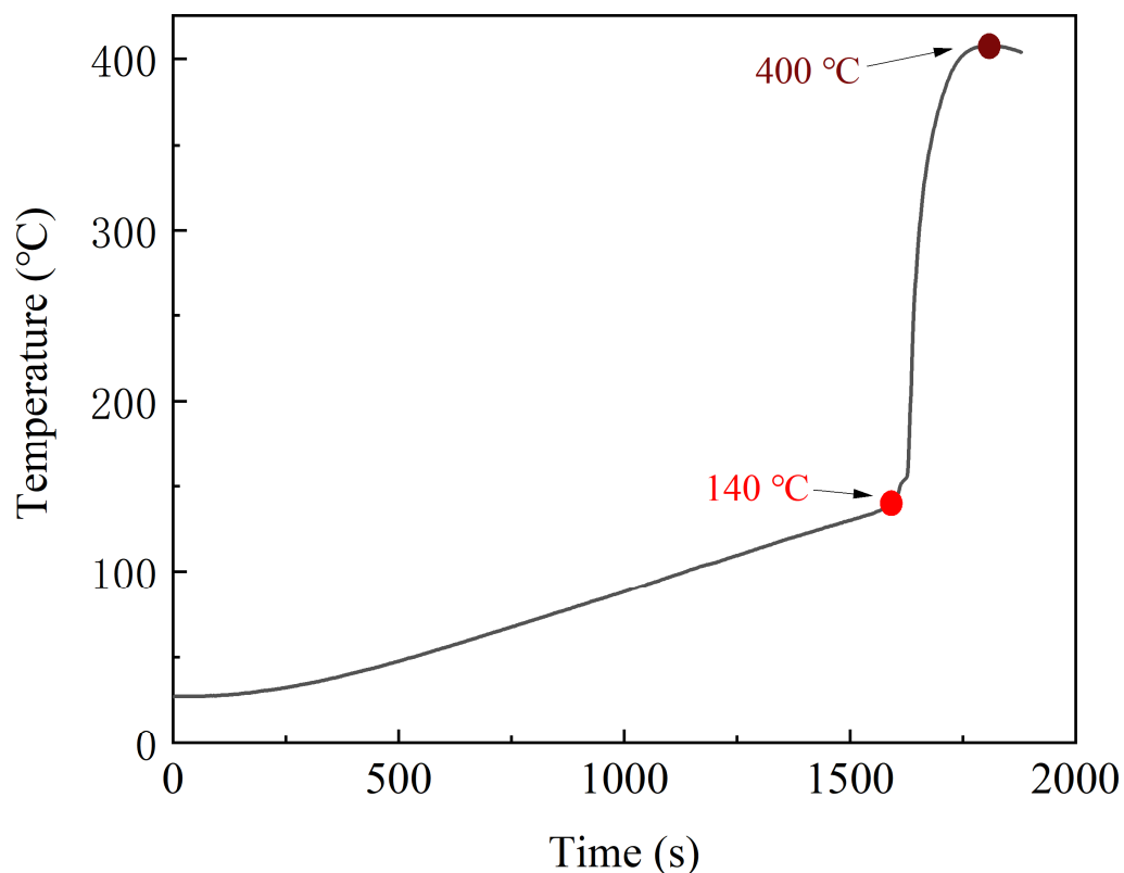
Figure 2. Battery thermal runaway temperature curve in Case 1.
