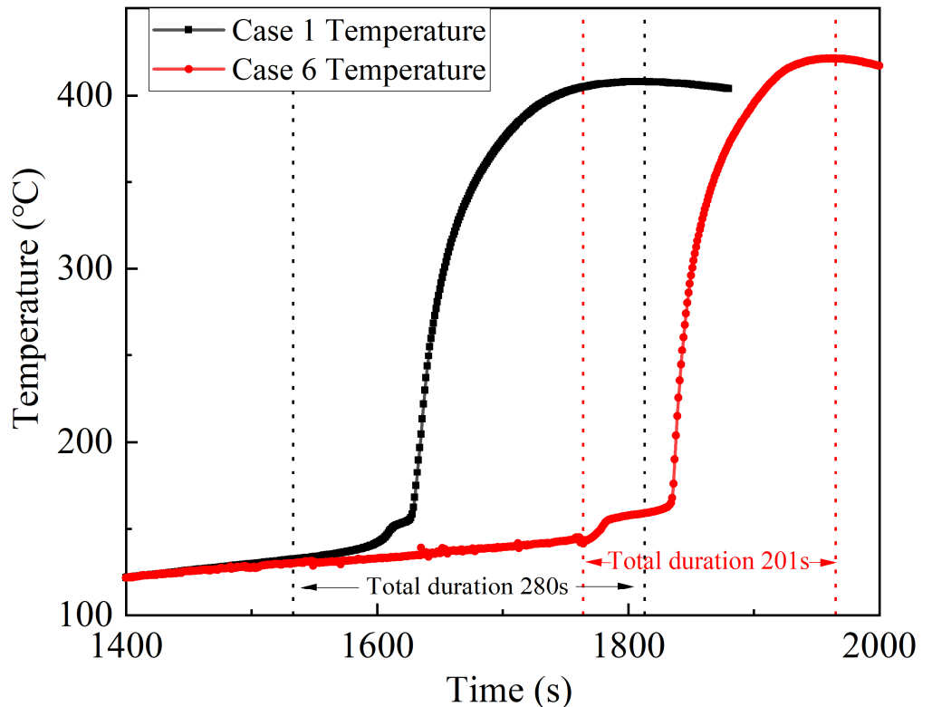
Figure 6. Variation curves of thermal runaway temperature of batteries in Cases 1 and 6.
