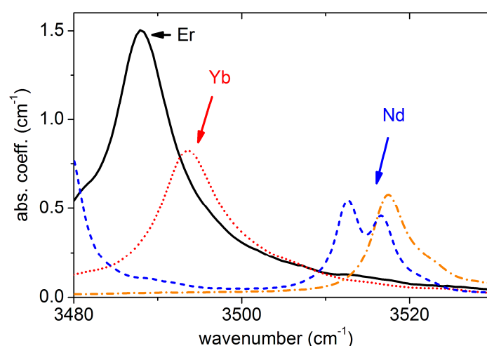
Figure 2. \text{OH}^- absorption bands in sLN crystals grown with \approx 0.44\text{ mol\% RE}_2\text{O}_3 (black continuous Er, red dotted Yb, and blue dashed Nd). The Czochralski grown sLN doped with 0.85 mol% \text{Nd}_2\text{O}_3 is also shown (orange dash-dot).
