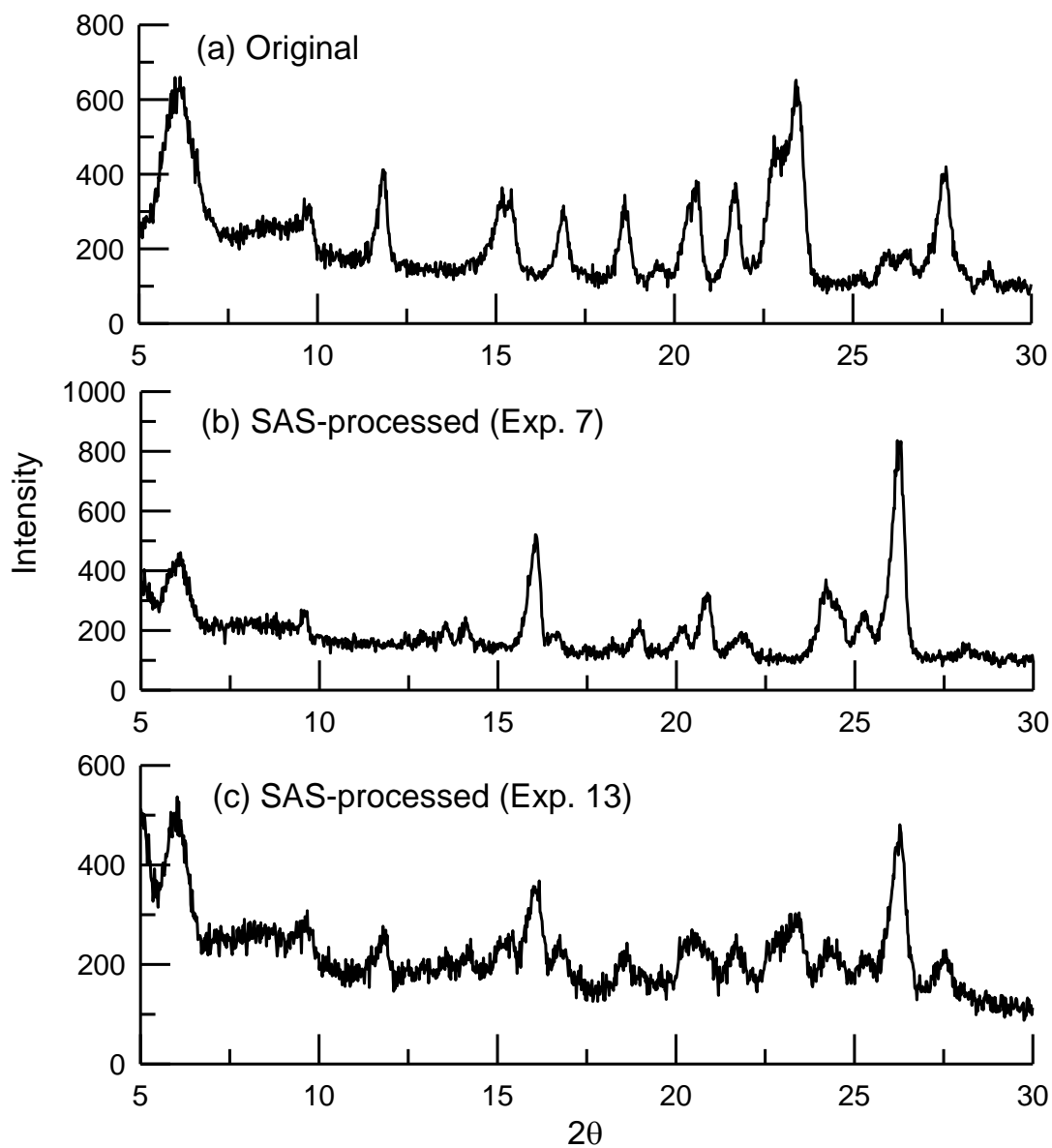
Fig. S2 PXRD results of sulfasalazine crystals: (a) original crystals as form I, (b) form II crystals obtained from Exp. 7, and (c) A form I + II mixture obtained from Exp. 13.
