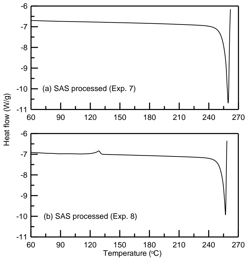
Fig. S1 DSC results of sulfasalazine crystals: (a) crystals obtained from Exp. 7 and (b) crystals obtained from Exp. 8.
