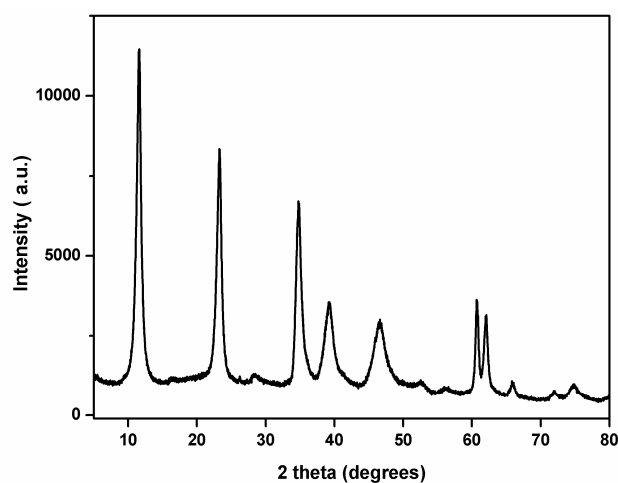
Figure S1 XRD pattern of LDH.
