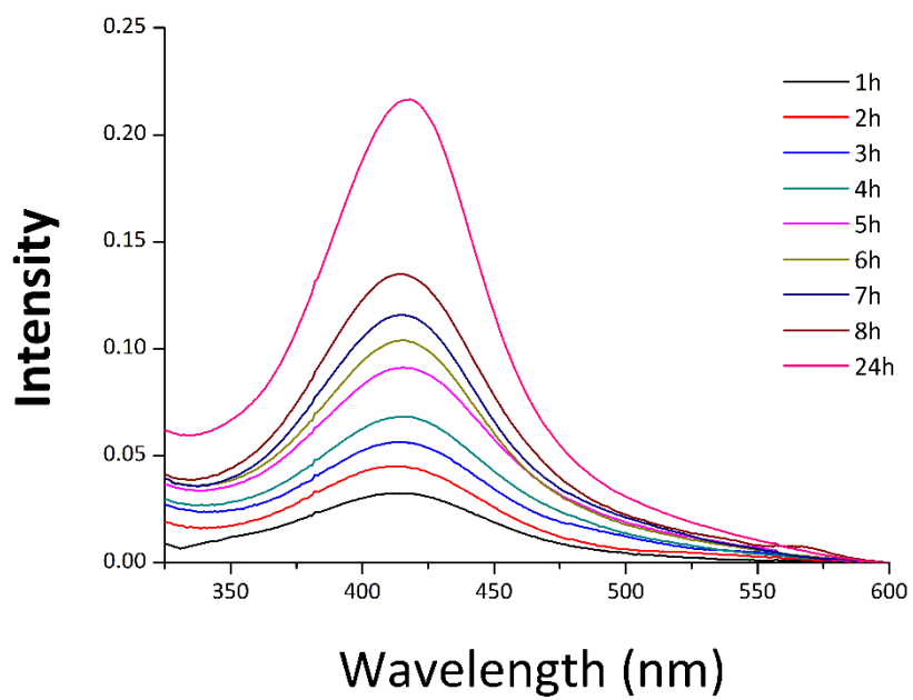
Figure S2 UV-vis analyses of the surrounding solution over time for sample A
