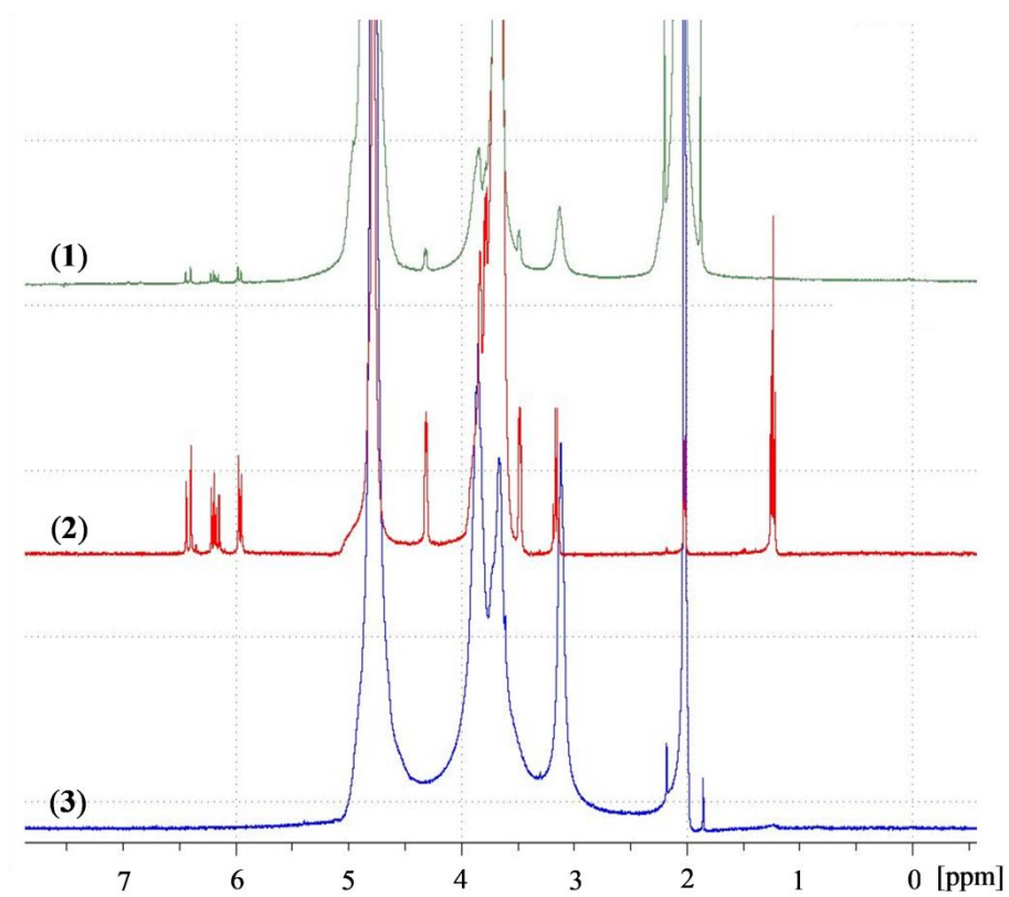
Figure S2. ^1\text{H} NMR spectra of (1) ACS, (2) PEGDA and (3) CS in \text{D}_2\text{O} .
