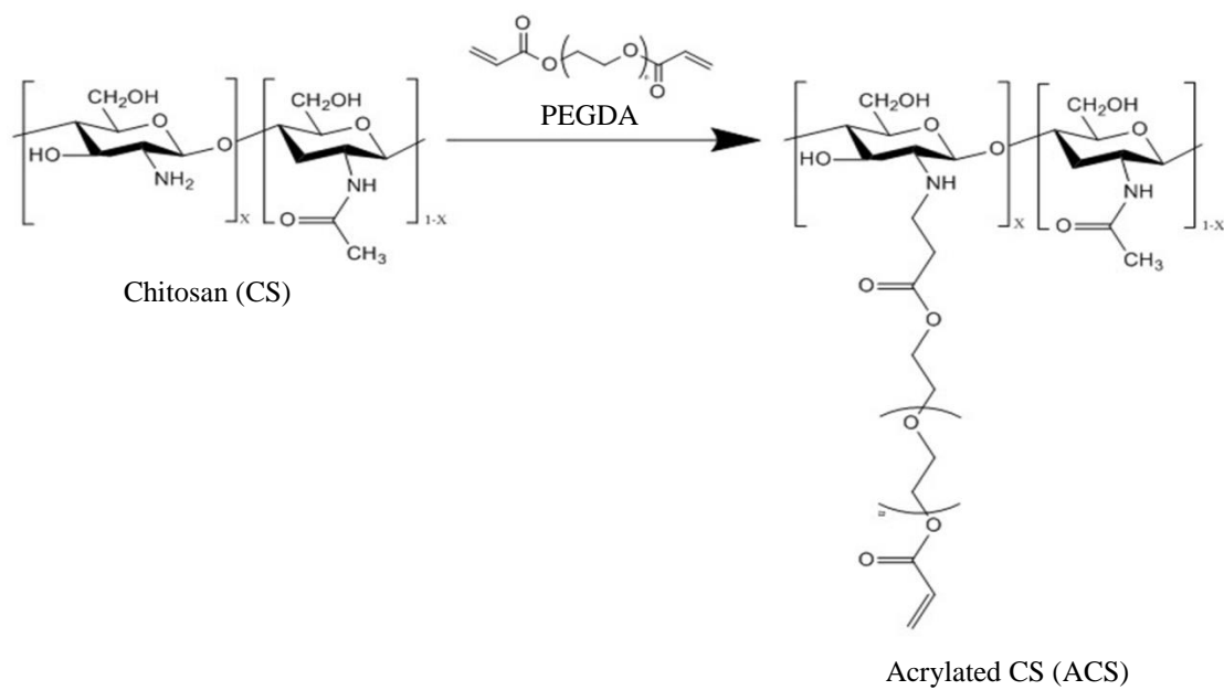
Figure S1. The molecular structure of ACS.
