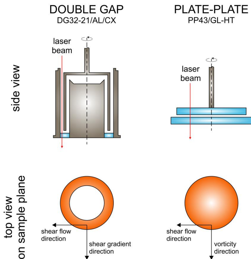
Figure S2. Schematic presentation of measurement systems: double gap and plate-plate. The top view on sample plane shows different measurement planes.
