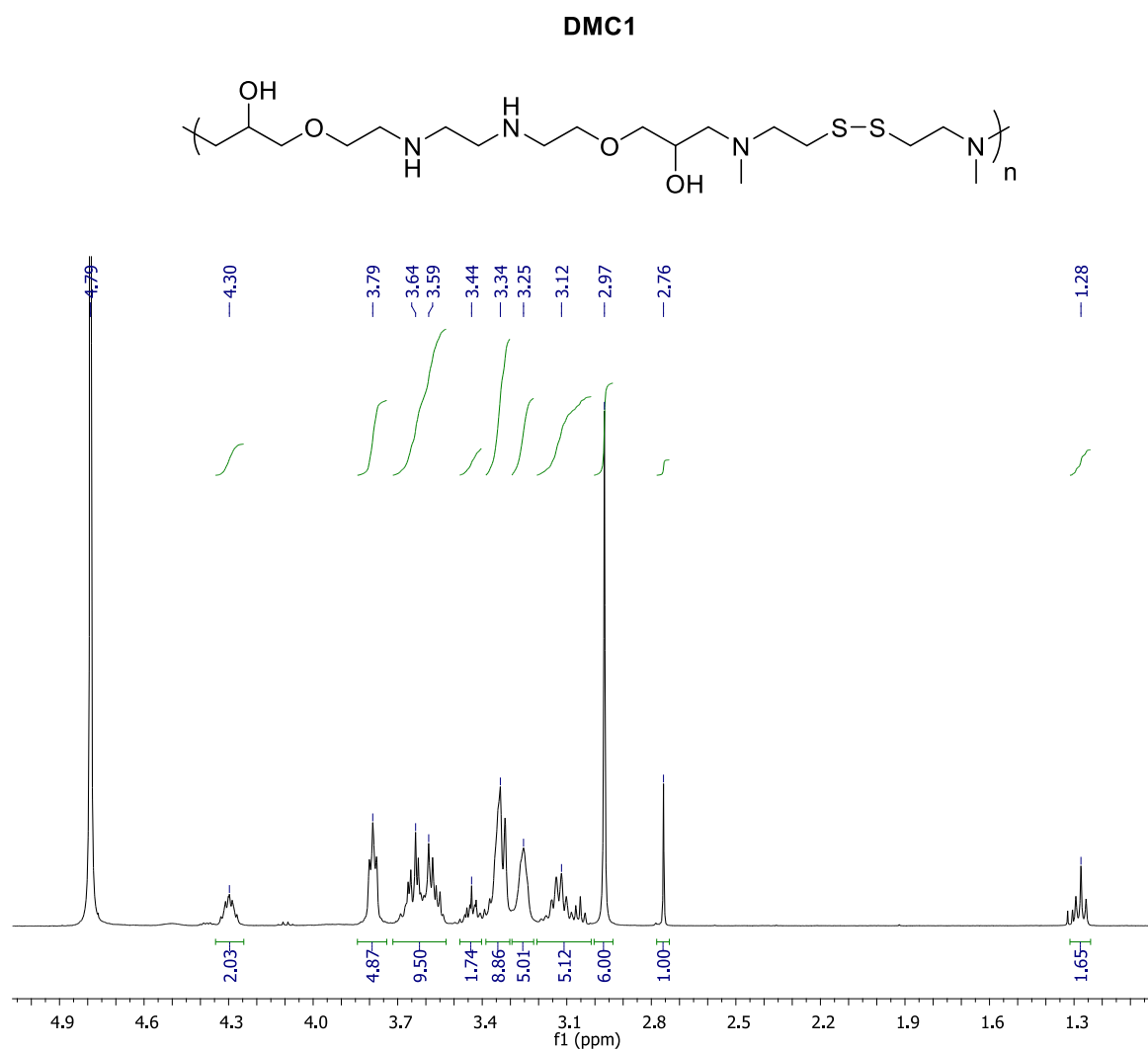
Figure S1. 1 H-NMR spectrum of DMC1 in D 2 O.
