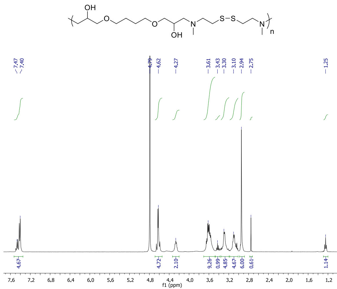
Figure S6. 1 H-NMR spectrum of DMC6 in D 2 O.
