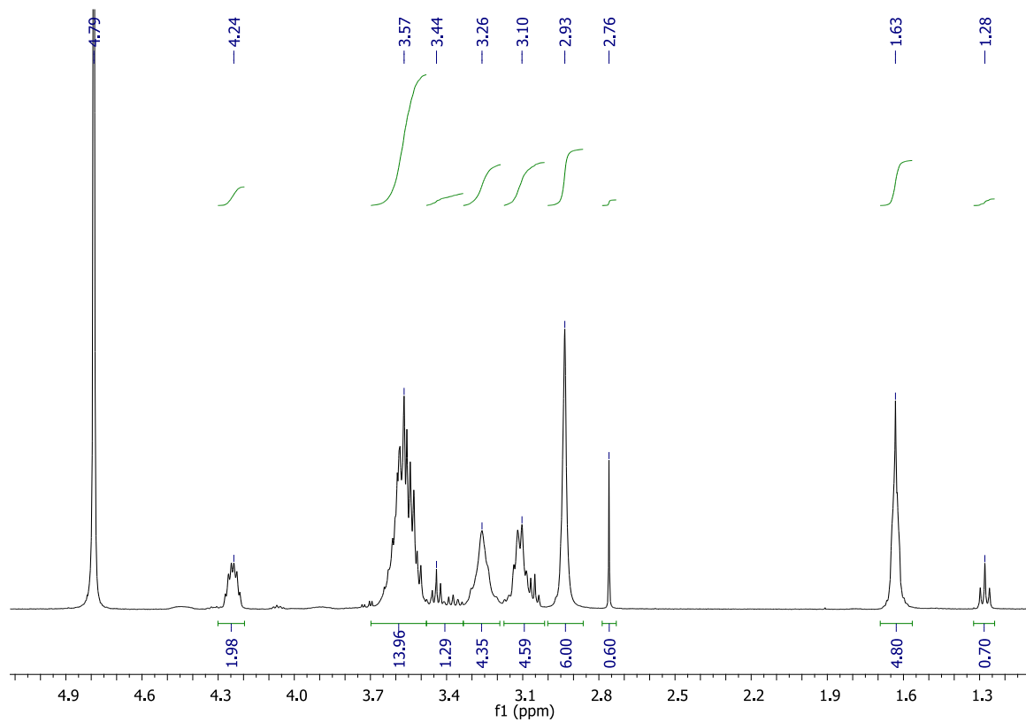
Figure S5. 1 H-NMR spectrum of DMC5 in D 2 O.
