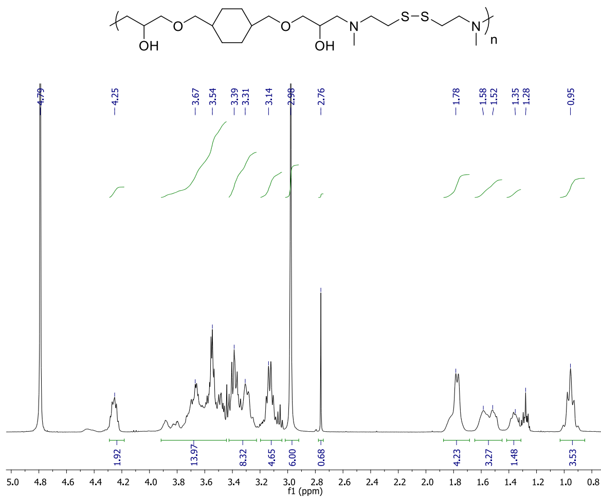
Figure S3. 1 H-NMR spectrum of DMC3 in D 2 O.
