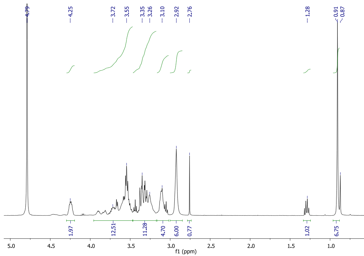
Figure S4. 1 H-NMR spectrum of DMC4 in D 2 O.
