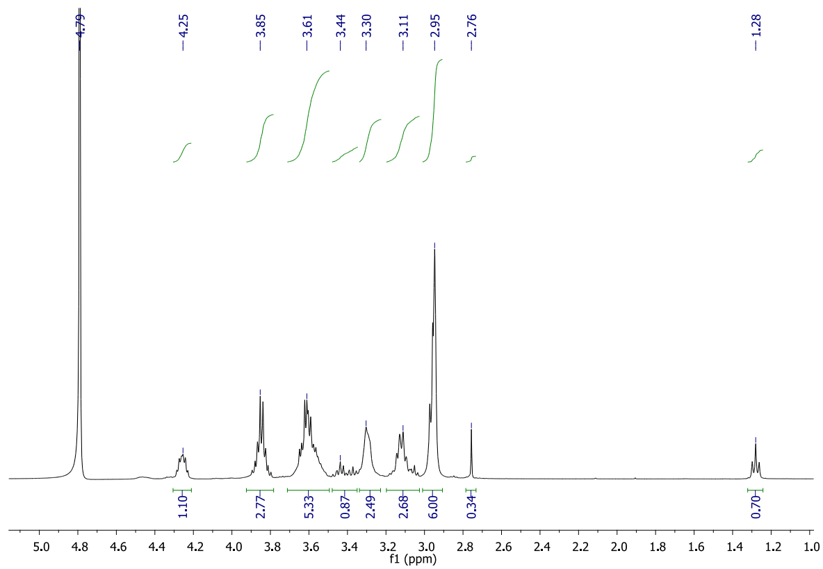
Figure S2. 1 H-NMR spectrum of DMC2 in D 2 O.
