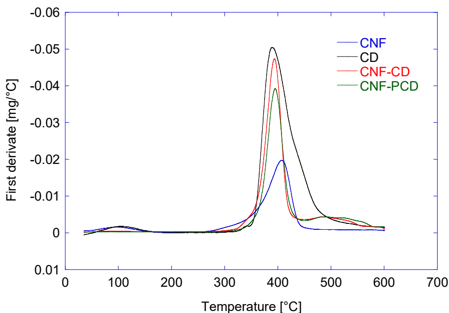
Figure S1. First derivative of thermogravimetric analysis of the CNF, CD, and the modified cellulose nanofibrils (CNF-CD and CNF-PCD).
