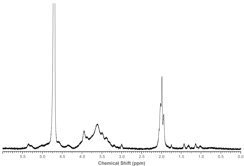
Figure S1. 1 H NMR spectrum of AC.
