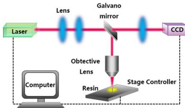
Figure 1. Schematic diagram of a DLW system.
