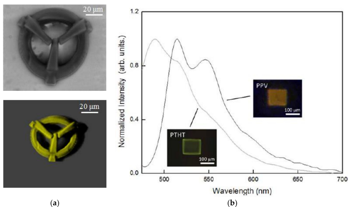
Figure 26. (a) The SEM and fluorescence images of PPV-doped microstructure; and (b) photoluminescence spectra of the same direct writing structure before (PTHT doped) and after thermal conversion (PPV doped) [123].
