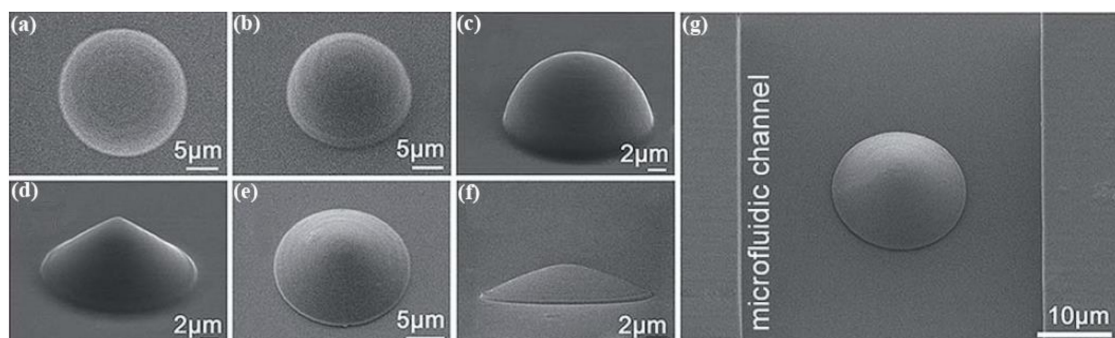
Figure 9. The SEM images from different view angles of (a–c) Spherical microlens and (d–f) aspheric hyperboloid microlens; and (g) SEM image of the microfluidic channel integrated with microlens [65].
